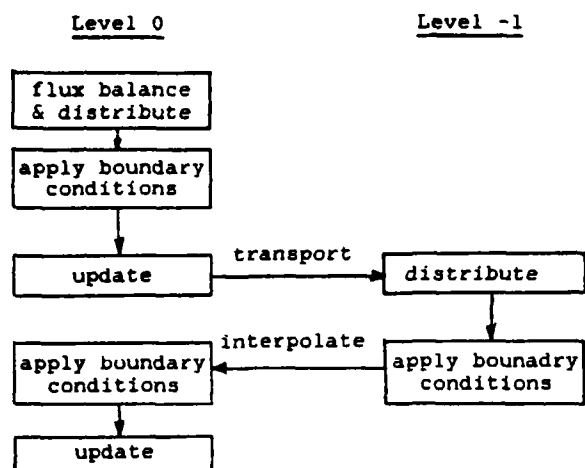
Figure 7. Ni multiple-grid cycle.
