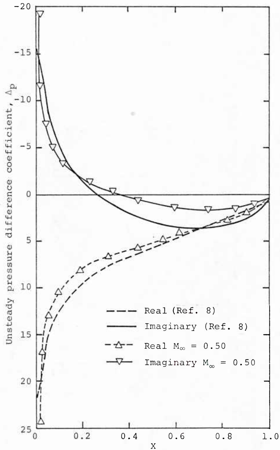
Figure 4.- Unsteady pressure distribution around a flat plate in torsion; M_\infty = 0.5 , G = 1.0 , \nu = 1.0 .
