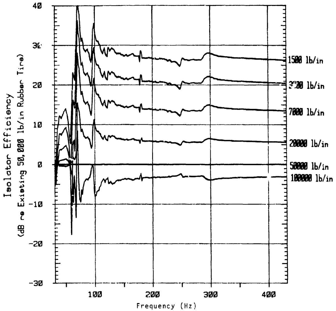
Figure 3.1 Calculated Isolator Efficiency for Compliant Roadwheel. Family of Curves are for Various Tire Spring Rates.
