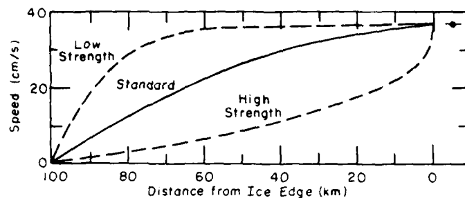
Fig. 4. Variable viscosity cases. The symbol \leftrightarrow shows free-drift value.
