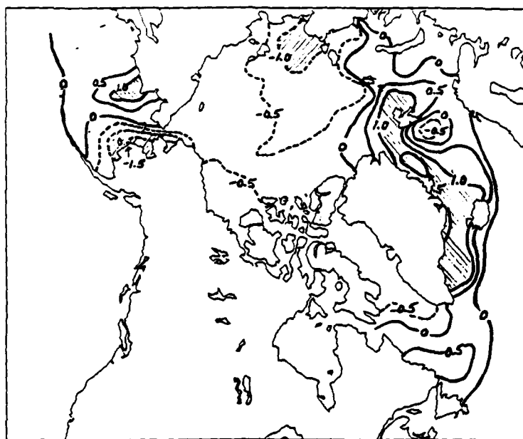
Fig. 2. 20-year simulation for (a) annual net ice growth (m) and (b) thickness changes associated with ice transport. Regions in which magnitudes of annual values exceed 1.0 meter are shaded. Positive values indicate net growth, negative values indicate net melt.
