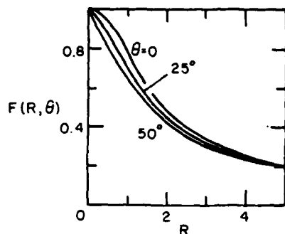
Fig. 1. The function F in the free-drift solution.
