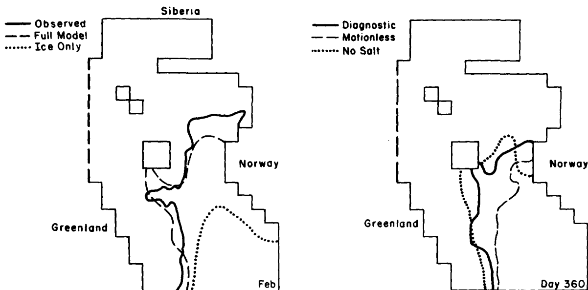
(b) Simulated 0.05 m thickness contours for day 360 for the full model, a "motionless" ocean model, and a coupled ice/ocean model with no salt fluxes due to ice freezing and melting. The "motionless" model and the no-salt simulations were run for only 1 year and were initialized to ice thickness and ocean fields at the end of the fourth year of the full diagnostic model simulation.
