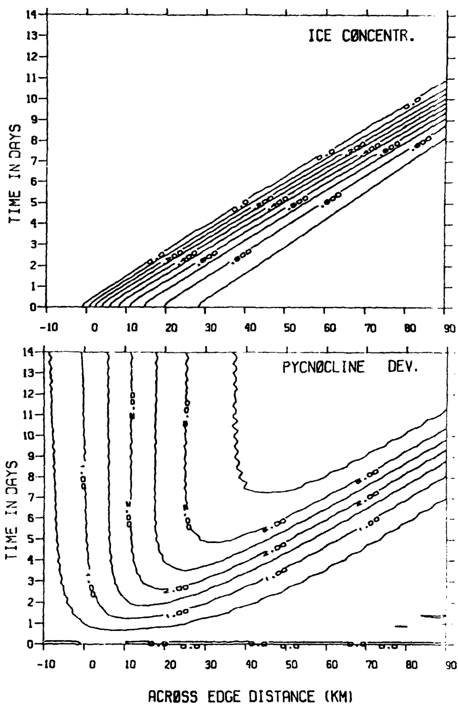
Fig. 3. (a) Same as Figure 2. In this case we have only one ice edge. (b) Solid curves show the time and space dependence of the pycnocline deviation (in m), away from its equilibrium position. Time in days is shown along the vertical axis. The across-edge distance (in km) is measured from the ice edge. The contour interval is 0.5.
