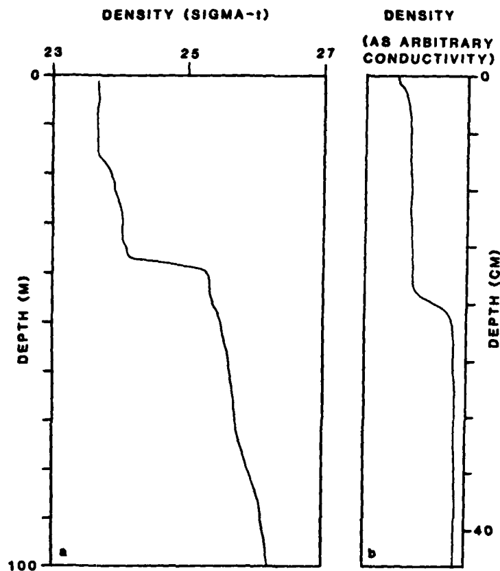
Fig. 2. Vertical profiles showing (a) the vertical distribution of density in the summer Beaufort Sea MIZ, and (b) the vertical distribution of density (saliency expressed here as conductivity) used in the actual laboratory experiment.
