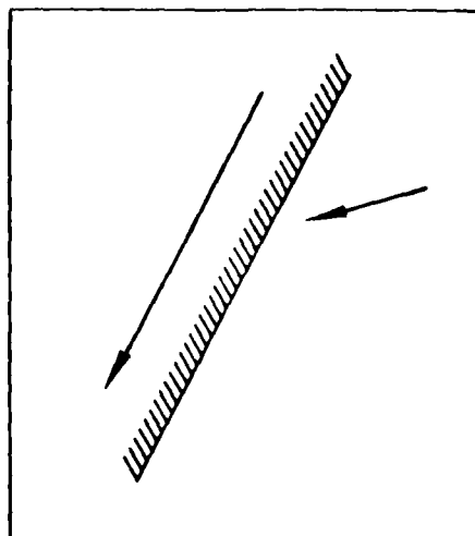
Fig. 1a. Expected wind direction in the vicinity of the ice edge (from Sigtryggsson and Stefansson, 1969).
