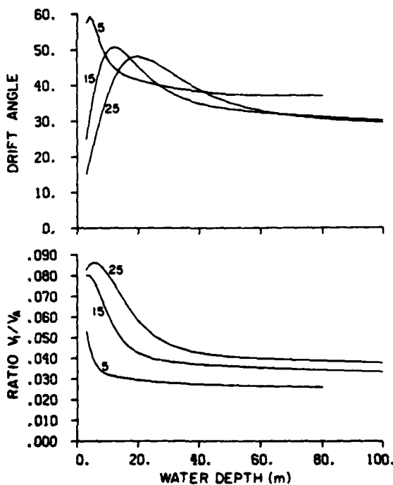
Fig. 1. The speed ratio and turning angle as a function of water depth for wind speeds of 5, 15, and 25 m/s.
