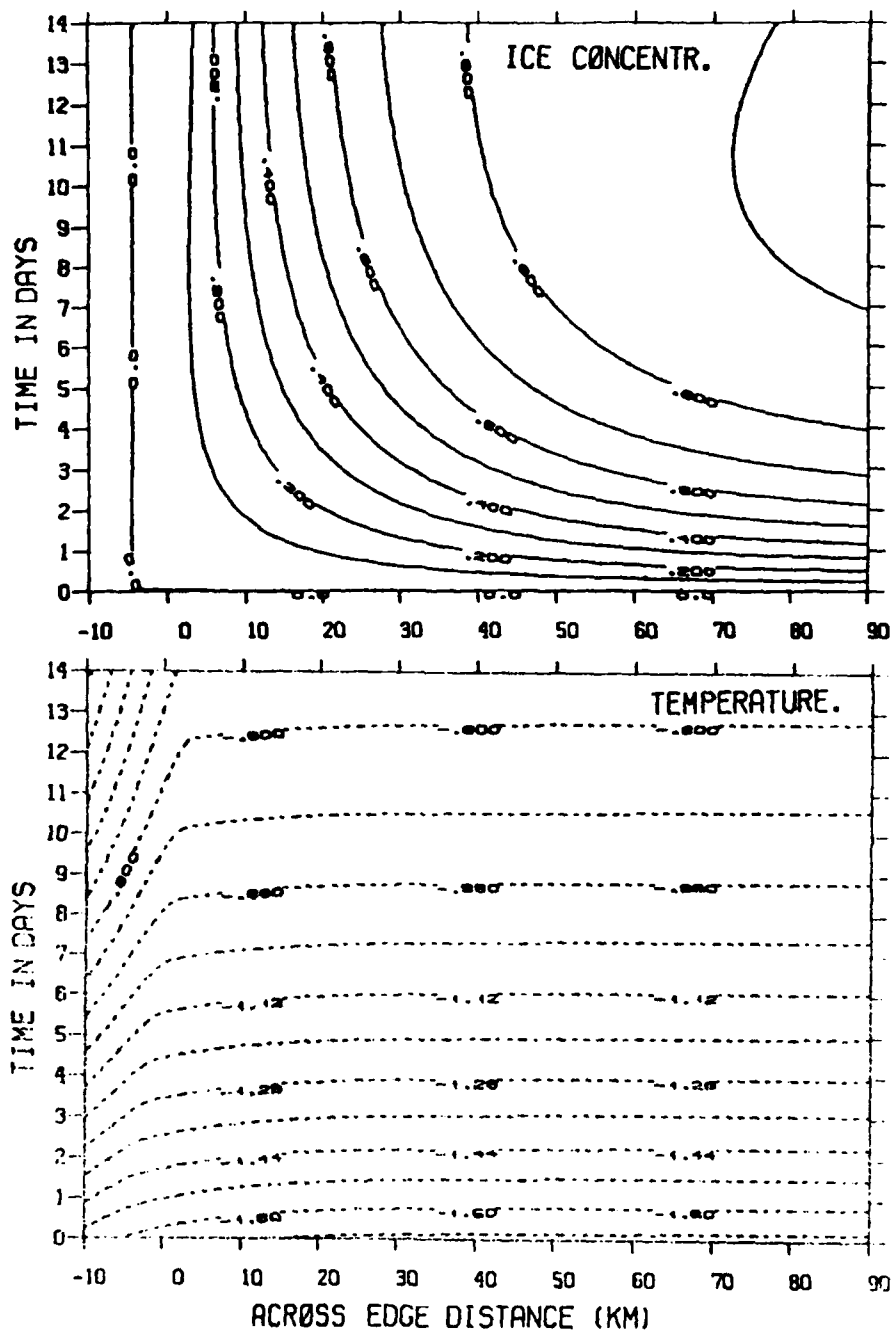
Fig. 2. (a) Same as Figure 1. In this case we have used the thermodynamic model alone. Initially the ice concentration was zero. (b) Dashed curves depict the mixed-layer temperature in ^{\circ}\text{C} . The vertical and horizontal axes are the same as in Figure 1. The contour interval is 0.08.
