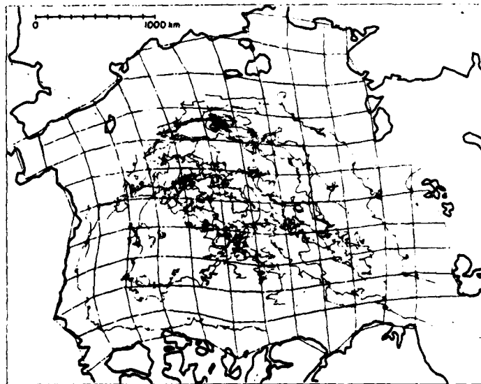
Fig. 1a. Trajectories of various research stations (1893-1972) (Hastings, 1971).
