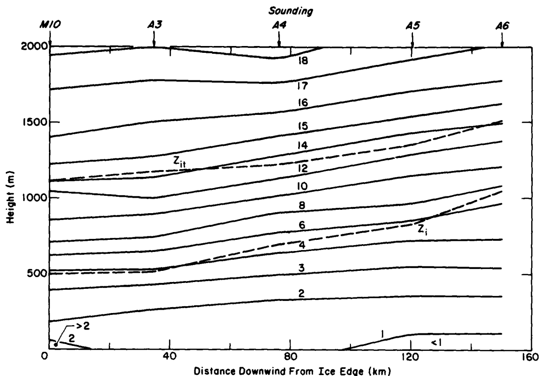
Fig. 3. Contours of potential temperature in °C along the ship track. Z_i indicates the height of the inversion, and Z_{ii} shows the top of the inversion layer.
