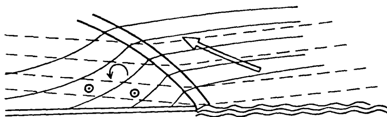
Fig. 1b. A vertical cross-section of the atmosphere above the leading edge of the ice pack viewing to the north. Solid lines are isotherms, dotted lines are isobars. The double line represents the frontal boundary. Currents blowing toward the viewer are indicated by a circle enclosing a point (from Sigtryggsson and Stefansson, 1969).
