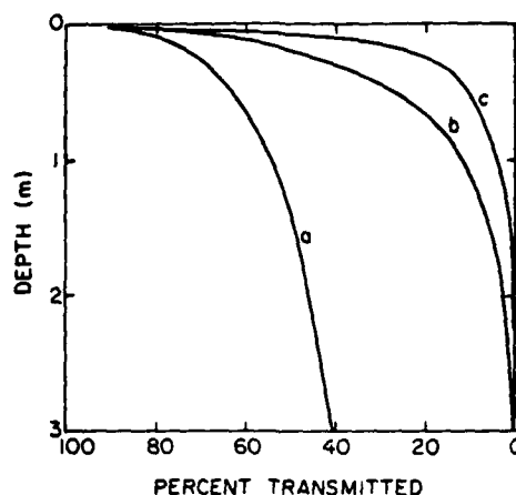
Fig. 1. Percent of incoming shortwave radiation transmitted by a) leads, b) blue ice, and c) white ice. Curves were calculated using the radiative transfer model of Grenfell (1979) and optical data from Grenfell and Maykut (1977).
