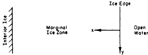
Fig. 1. The model MIZ and the coordinate system.
