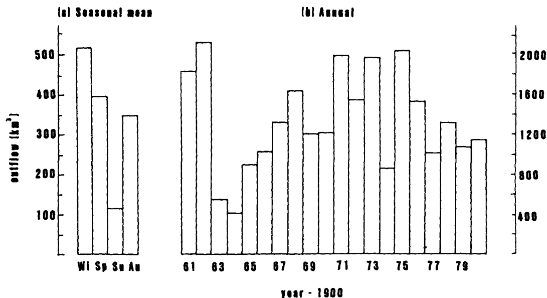
Fig. 3. Outflow of ice ( \text{km}^3 ) from central Arctic into East Greenland Sea. (a) 20-year seasonal means, where Wi = winter, Sp = spring, Su = summer and Au = autumn. (b) Annual totals.
