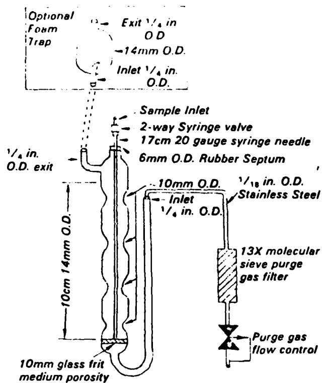
Figure 1. Purging device
