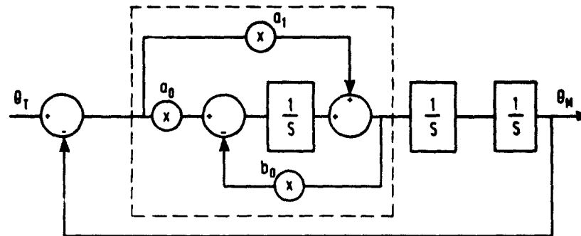
(b) STRUCTURE 2
