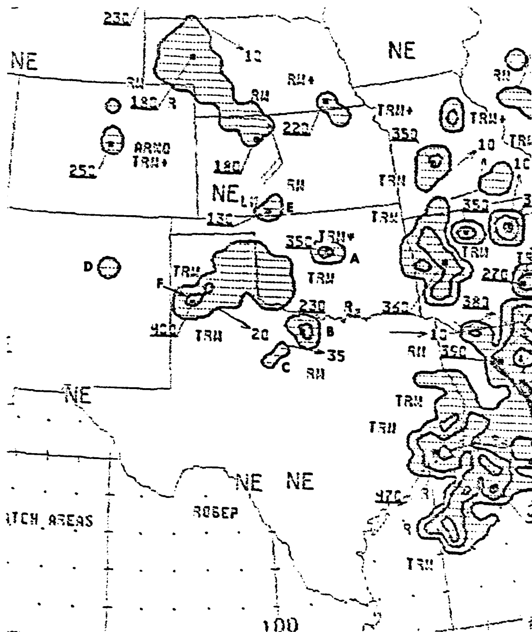
Fig. 44. Radar summary chart for 1735 GMT 26 June 1982. Shading indicates echo areas. Contours at echo intensities 1, 3, and 5; echo heights are in thousands of feet; cell movement given at end of arrows in knots; area and line movement given by pennant with full barb = 10 kt (U. S. Department of Commerce, 1981). Cells "A", "B", "C", "D", and "E" were along the second arc cloud. The strongest radar returns within the ACC are marked "F".
