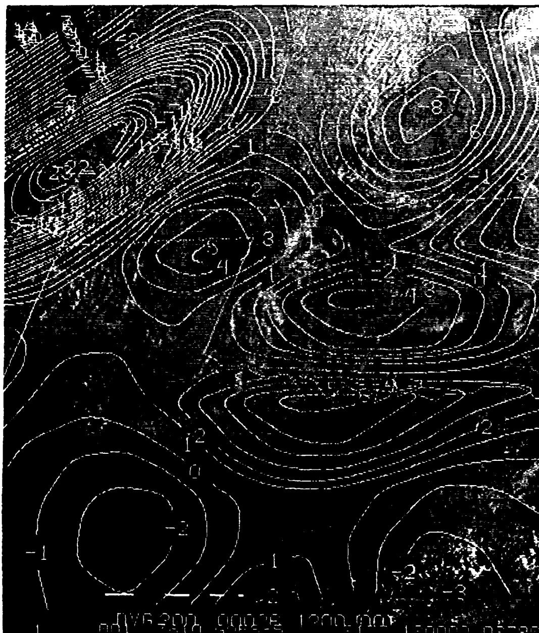
Fig. 30. 300 mb divergence overlaid upon GOES image for 1200 GMT 26 June 1982. Values are times 10^{-5} \text{ s}^{-1} .
