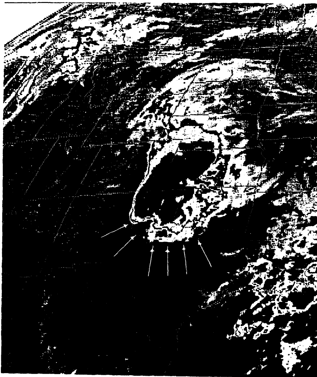
Fig. 21. GOES infrared image with MB enhancement at 1201 GMT 26 June 1982. The arrows point out the first arc cloud.
