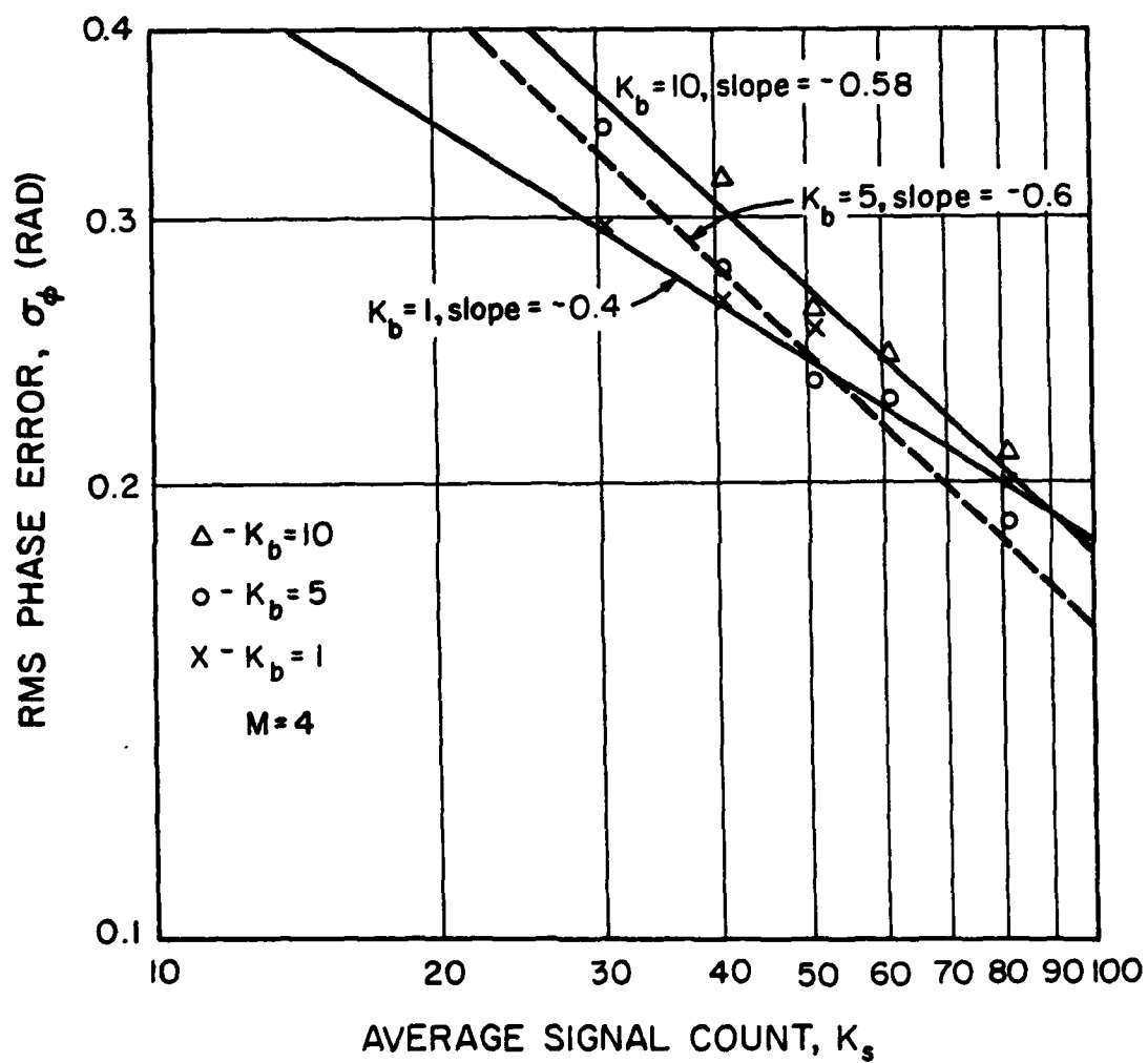
Figure 6.2. RMS phase error versus average signal count for M = 4 .
