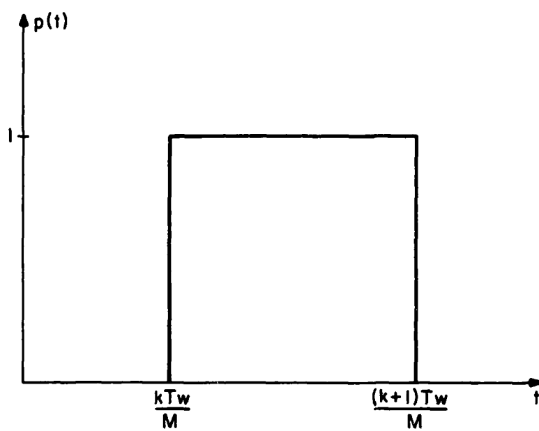
Figure 2.2. The received optical pulse shape, p(t) .
