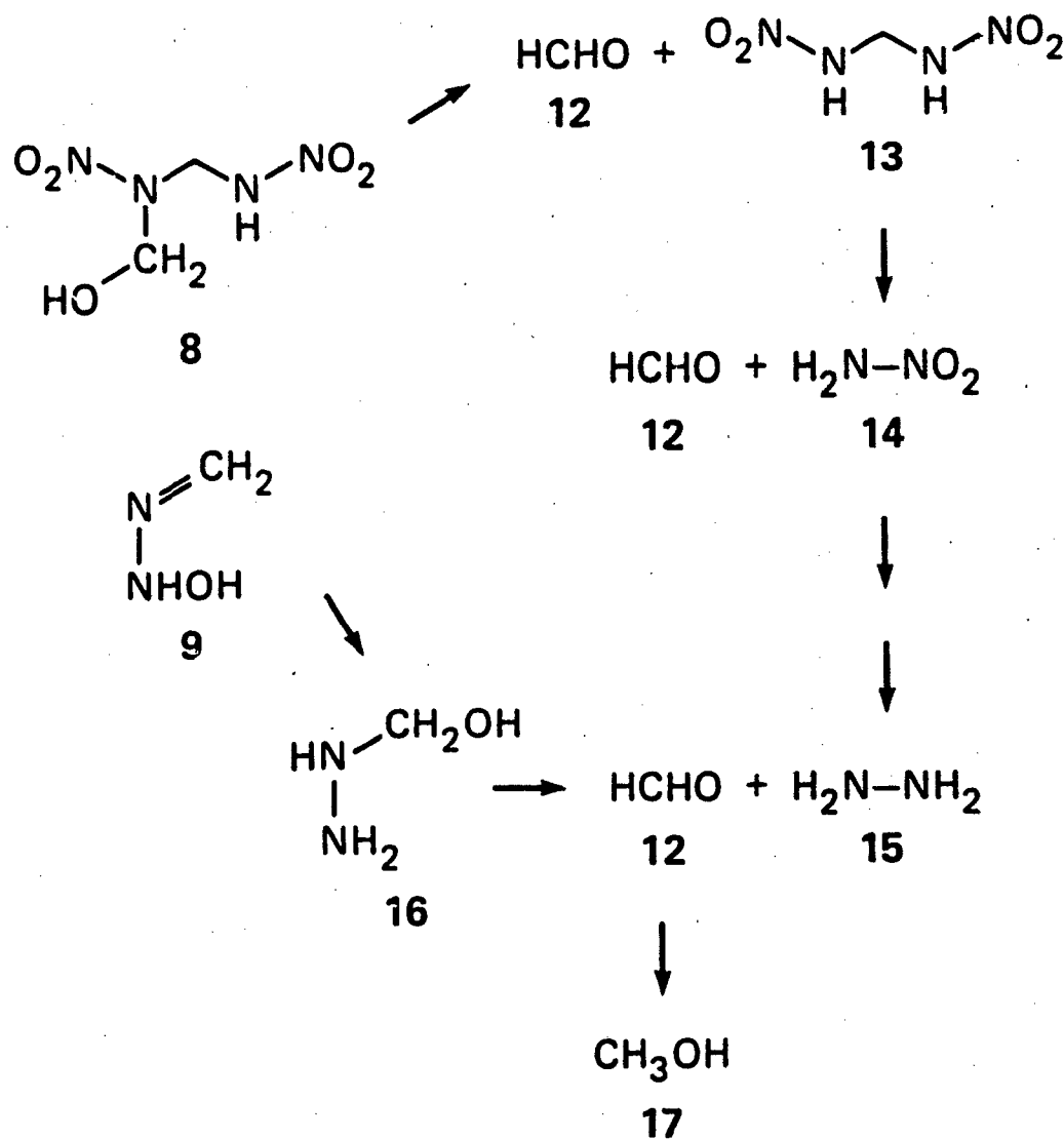
Figure 8.4. Final stages of proposed anaerobic degradation pathway of RDX-derived compounds. Compounds are: 8 = N-hydroxymethyl-methylenedinitramine; 9 = N-hydroxymethylene-hydrazone; 12 = \text{HCHO} ; 13 = methylenedinitramine; 14 = nitramide; 15 = hydrazine; 16 = hydroxymethylhydrazine; and 17 = methanol. From McCormick et al. 1981.
