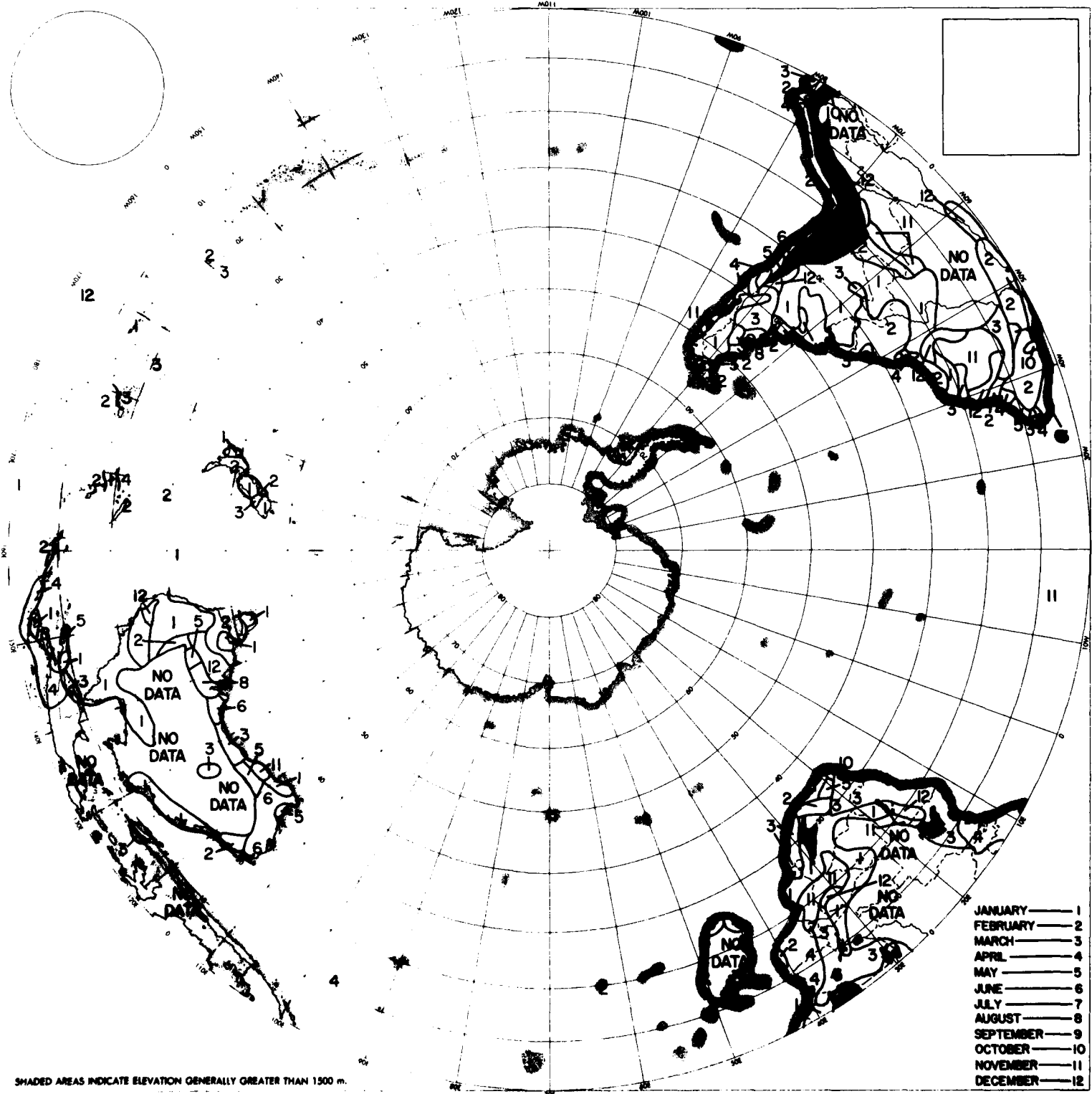
Figure 25. Month With the Highest 1-Min Rainfall Rates Equalled or Exceeded 0.05 Percent of the Time
