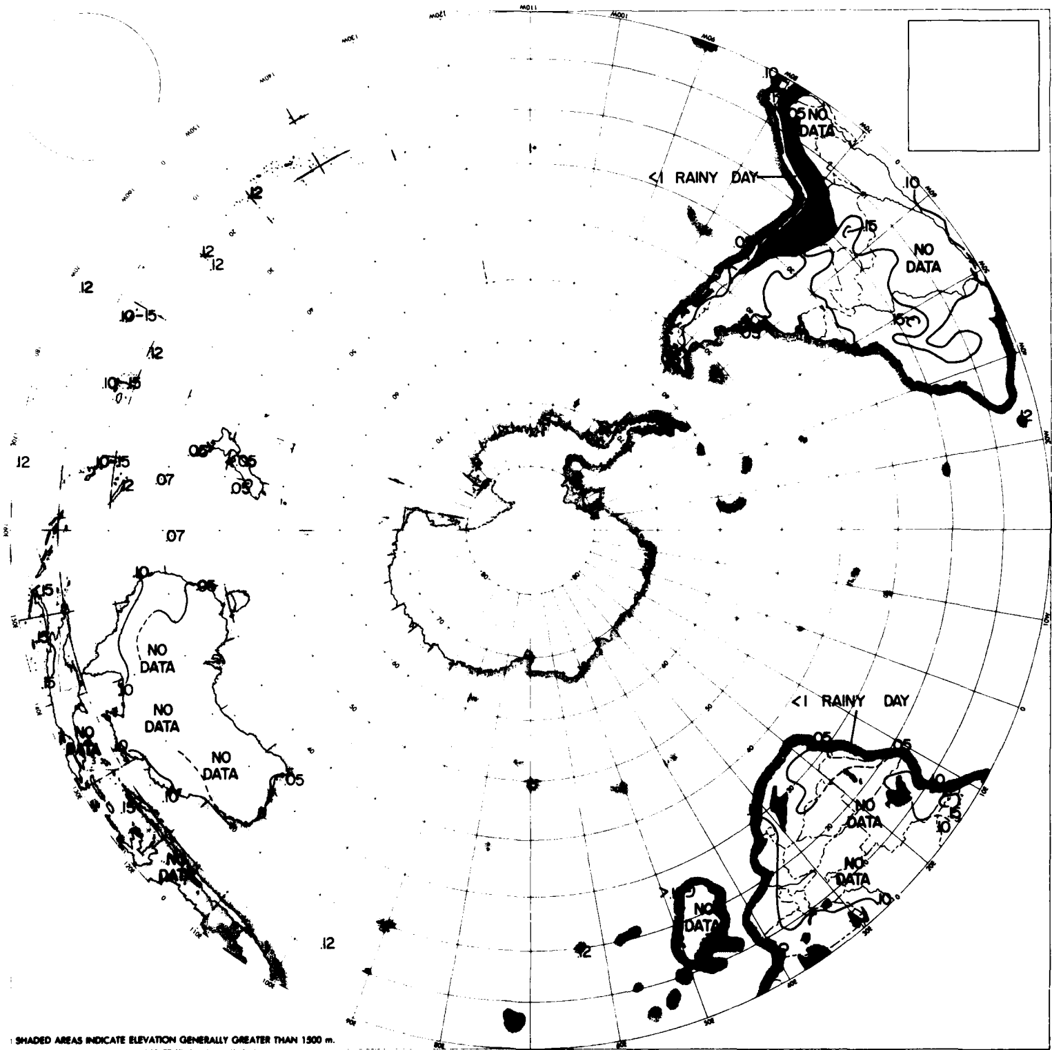
Figure 11. One-Min Rainfall Rate (mm/min) Equalled or Exceeded 1.0 Percent of the Time in April
