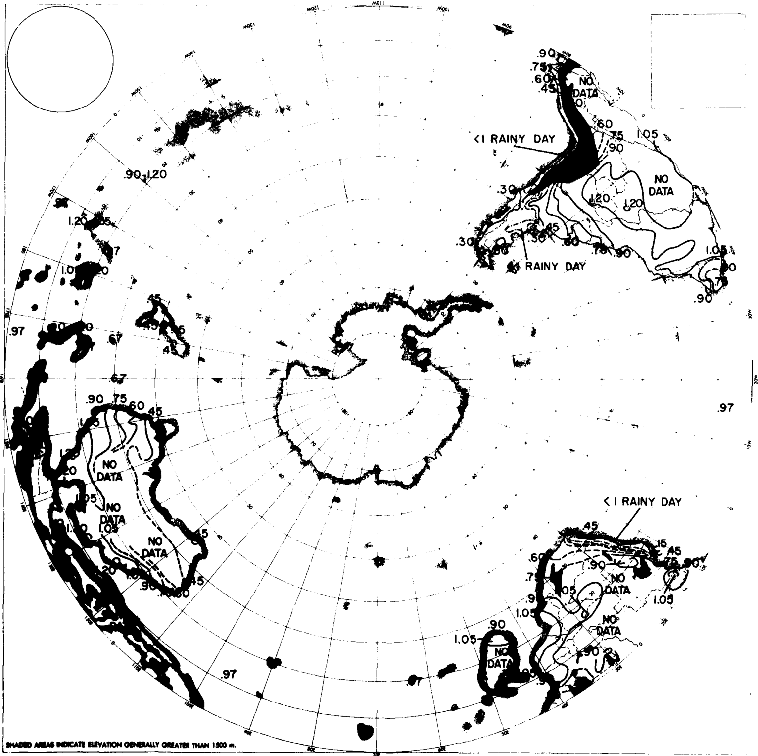
Figure 3. One-Min Rainfall Rate (mm/min) Equalled or Exceeded 0.05 Percent of the Time in January
