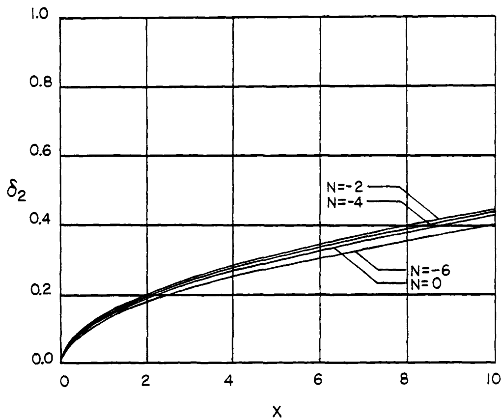
Figure 4.14 Momentum Thickness Versus Length X (inches) M = -2
