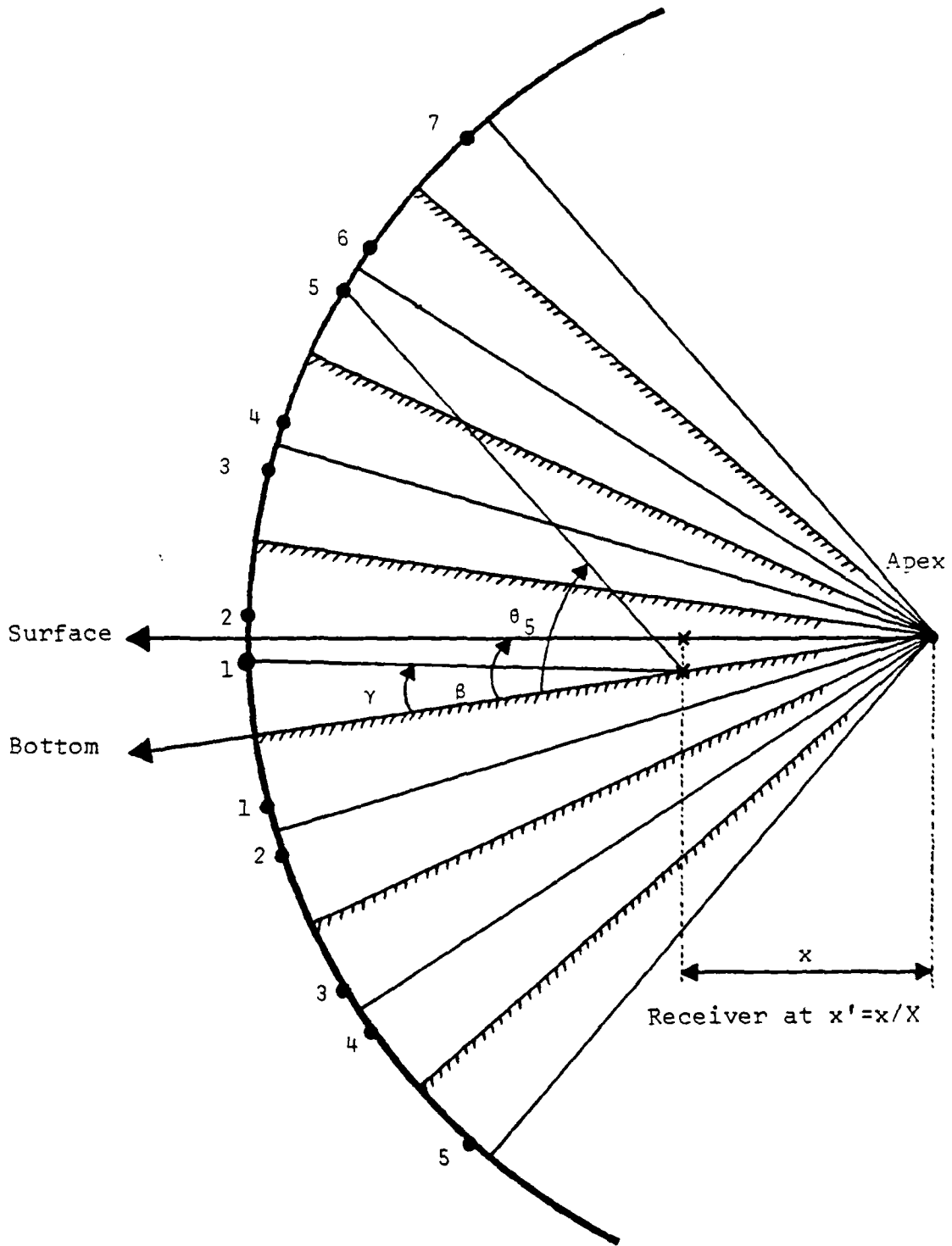
Figure 3 The Geometry of Image Solution
