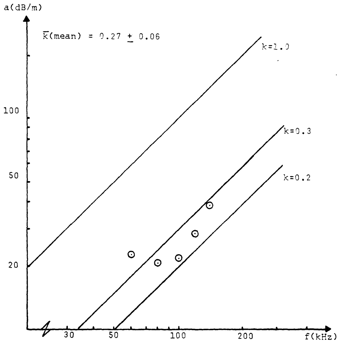
Figure 22 Attenuation in Sand
