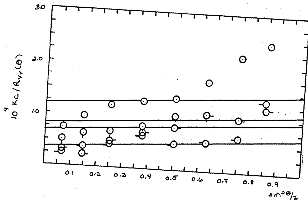
Figure 163: The aluncentrifuged Vv components of the integrated intensity light scattering of SPBO 80/MSA at 633 nm and 25.0°C. ○ 0.0511 g/dl ○ 0.0399 g/dl ◐ 0.0250 g/dl ⊗ 0.0099 g/dl
