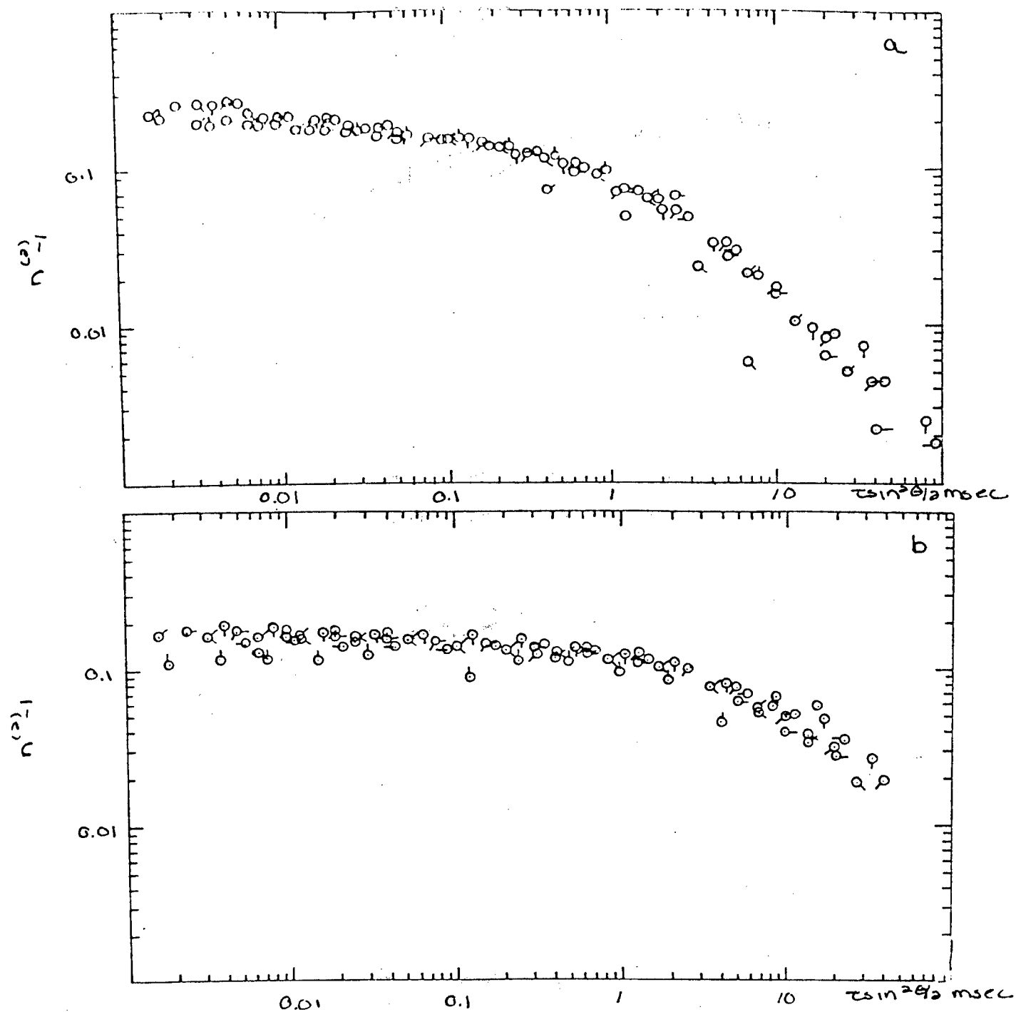
Figure 58: Intensity fluctuation light scattering n^2-1 versus \tau \sin^2 \theta/2 for centrifuged PBT 7 + salt at 514.5 nm and 25.0°C a) 0.0121 g/dl b) 0.0492 g/dl. \circ 45^\circ with pips clockwise to 135^\circ in 15^\circ increments.
