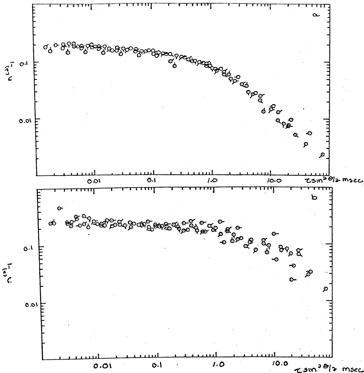
Figure 57: Intensity fluctuation light scattering I^{-1} versus r \sin^2 \theta/2 for PBT 7 + salt at 514.5 nm and 25.0^\circ\text{C} a) 0.0121 g/dl b) 0.0492 g/dl. \bigcirc 45^\circ with pips clockwise to 135^\circ in 15^\circ increments.
