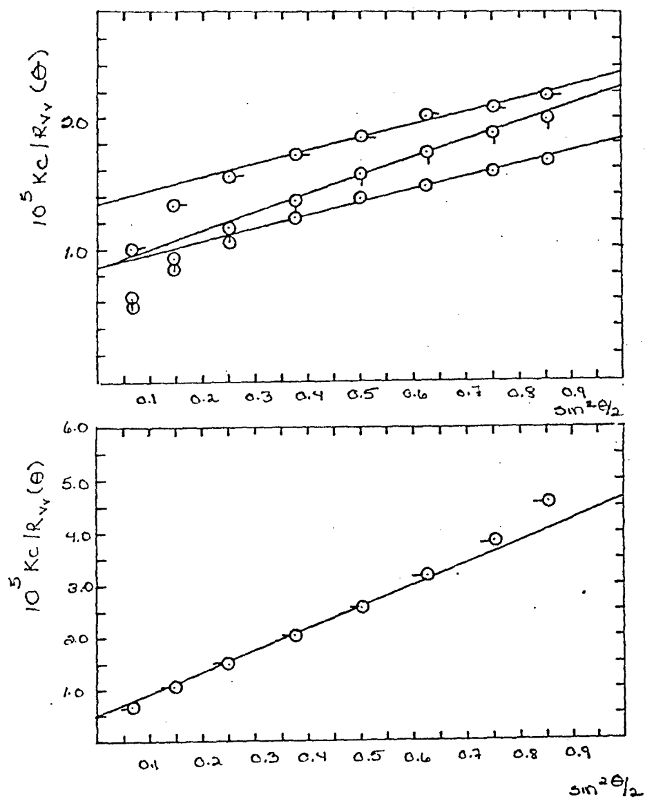
Figure 28: The centrifuged Vv component of the integrated intensity light scattering of PBT-PBO (75/25) in PPA/MSA at 514.5 nm and 25.0°C. \circ 0.0499 g/dl \circ 0.0381 g/dl \circ 0.0247 g/dl \circ 0.0102 g/dl
