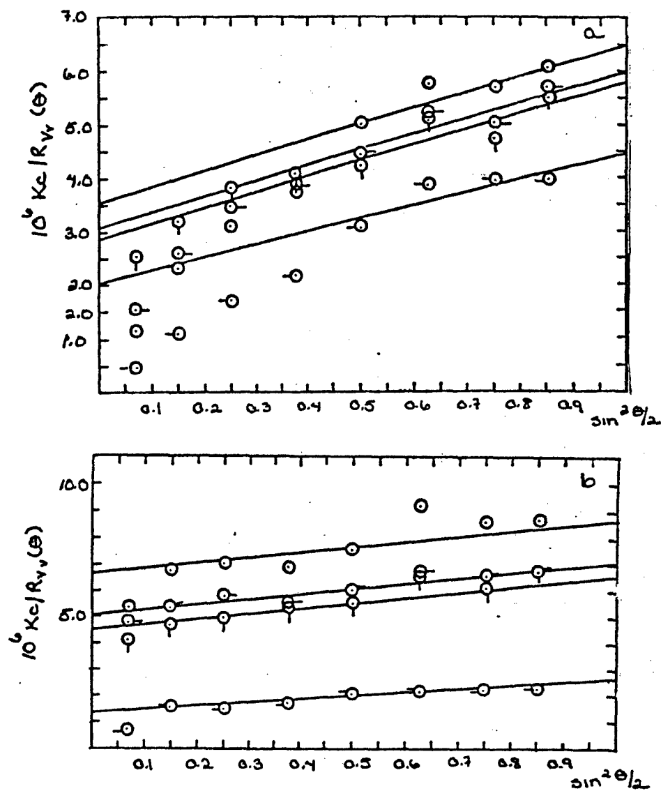
Figure 145: The a) uncentrifuged and b) centrifuged Vv components of the integrated intensity light scattering of SPBO 96/MSA at 514.5 nm and 25.0°C. O 0.0487 g/dl O- 0.0389 g/dl Q 0.0236 g/dl O- 0.0092 g/dl
