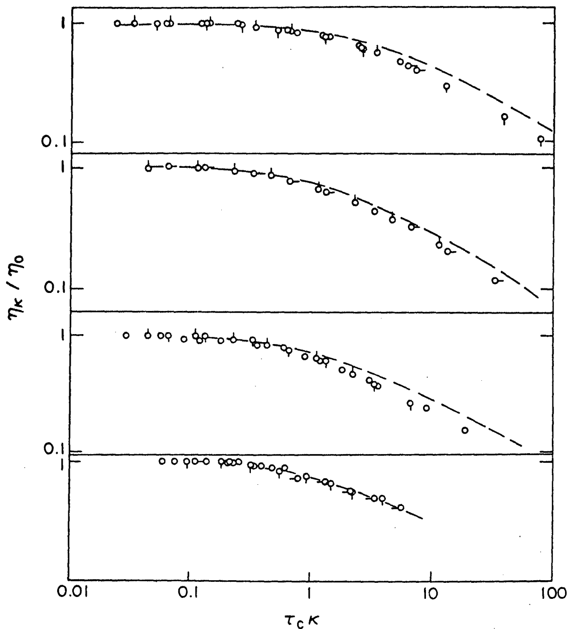
Figure 178: The reduced steady-state viscosity \eta_K / \eta_0 versus the reduced shear rate \tau_c K for solutions of PBT polymers in methane sulfonic acid. From top to bottom: PBT-72, 25.4 \text{ gkg}^{-1} (O, O, O for 24, 39, 55 C, resp.); PBT-72, 29.4 \text{ gkg}^{-1} , (O, O for 39, 58 C, resp.); PBT-72-R, 29.6 \text{ gkg}^{-1} (O, O, O for 23, 39, 58 C); PBT-43, 31.5 \text{ gkg}^{-1} (-O, O, O, O for 10, 14.5, 18, 23.5 C, resp.). The dashed curves represent the data for PBT-53, c = 25.5 \text{ gkg}^{-1} .
