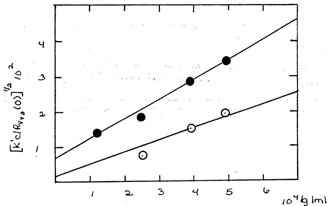
Figure 70: Concentration dependence of R_{vv,1} and R_{vv,2} , O uncentrifuged and ● centrifuged for solution of PBT 7 + salt at 25.0°C
