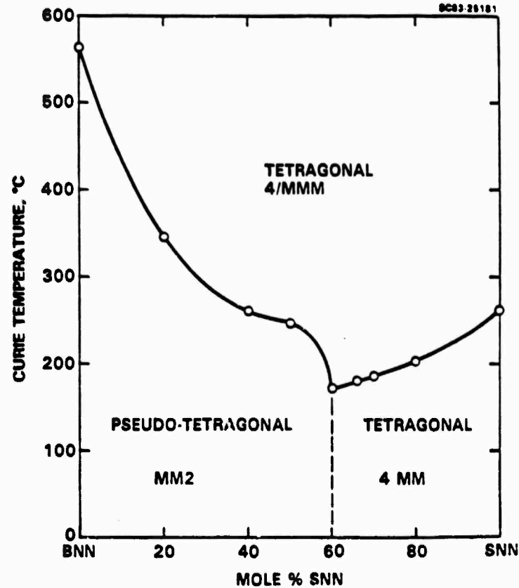
Fig. 6 Morphotropic phase boundary conditions for the system BNN-SNN.
