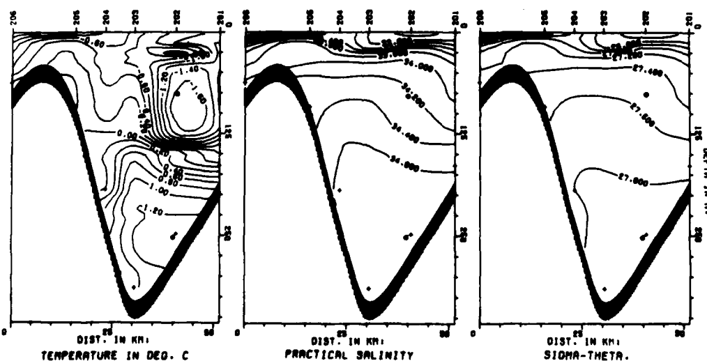
Fig. 4. A temperature, salinity and density section across the strait between Nordaustlandet and Kvitøya. The upper numbers identify the oceanographic stations. The deepest observations are marked with crosses and the positions of the current meters with black dots.
