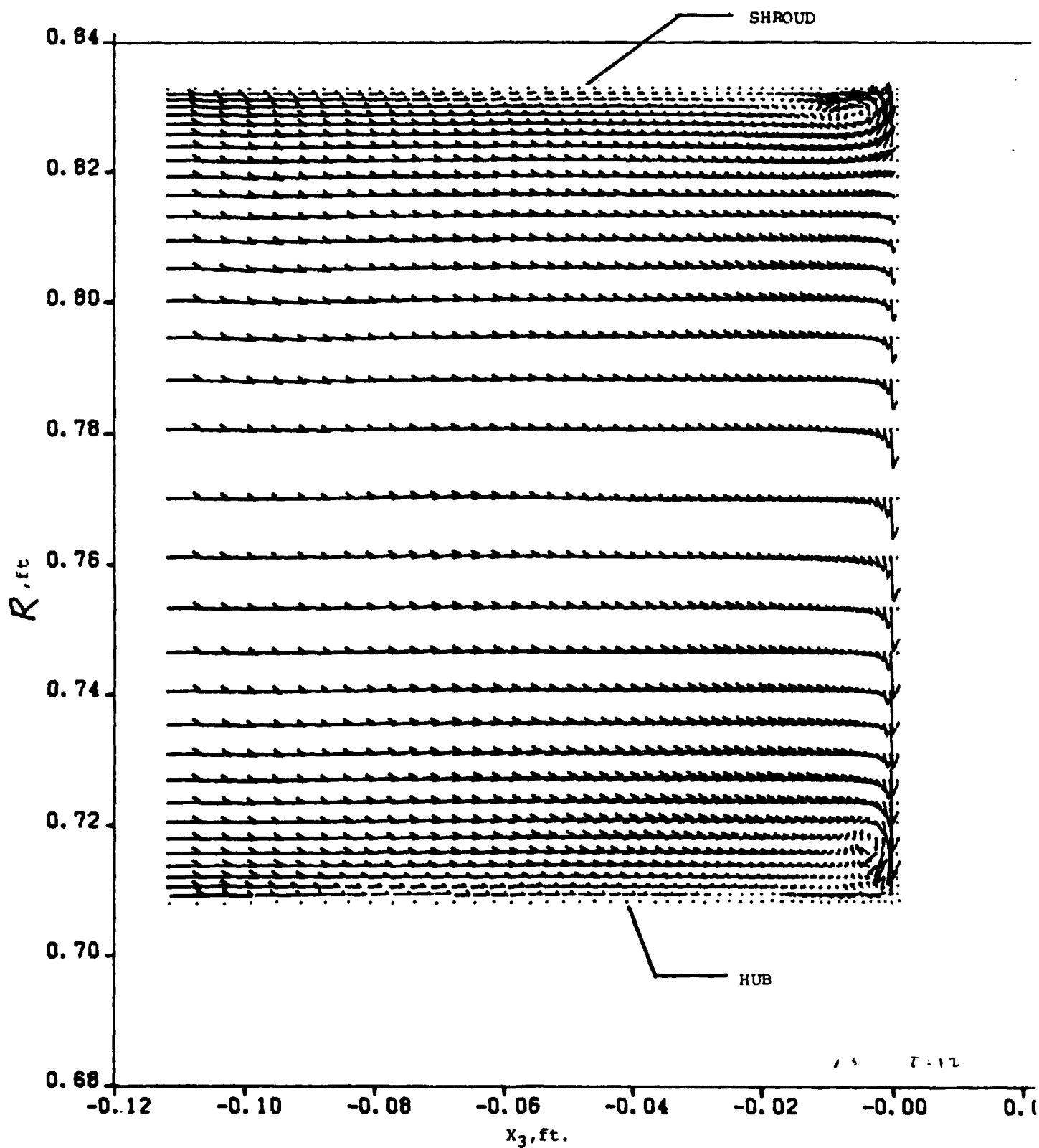
Figure 13. Velocity vector plot of the meridional flow field at z = -.1712269 radians; T=1.20
