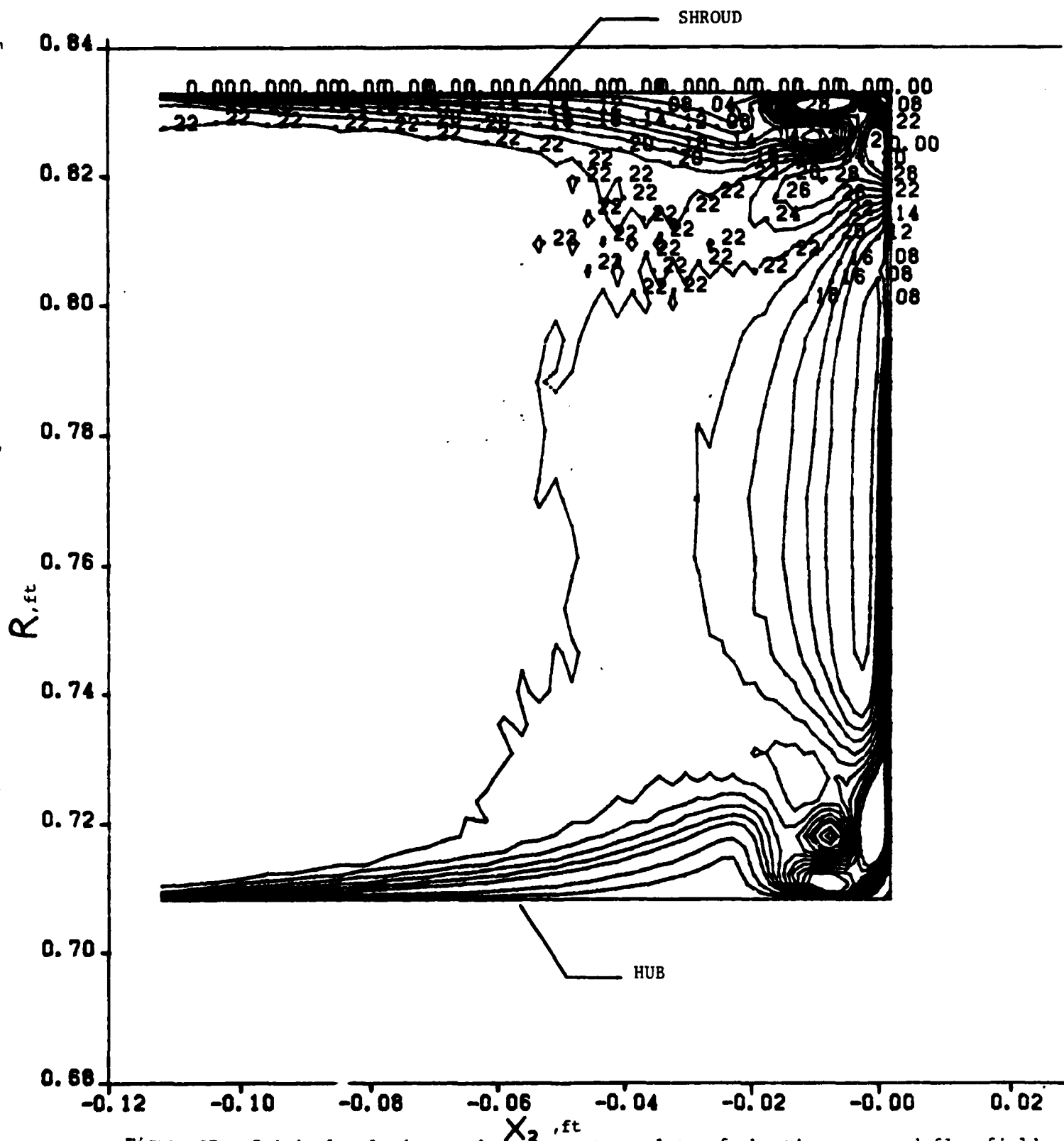
Figure 27. Critical velocity ratio X_3 contour plots of the time-averaged flow field at \alpha = -0.1660508 radians
