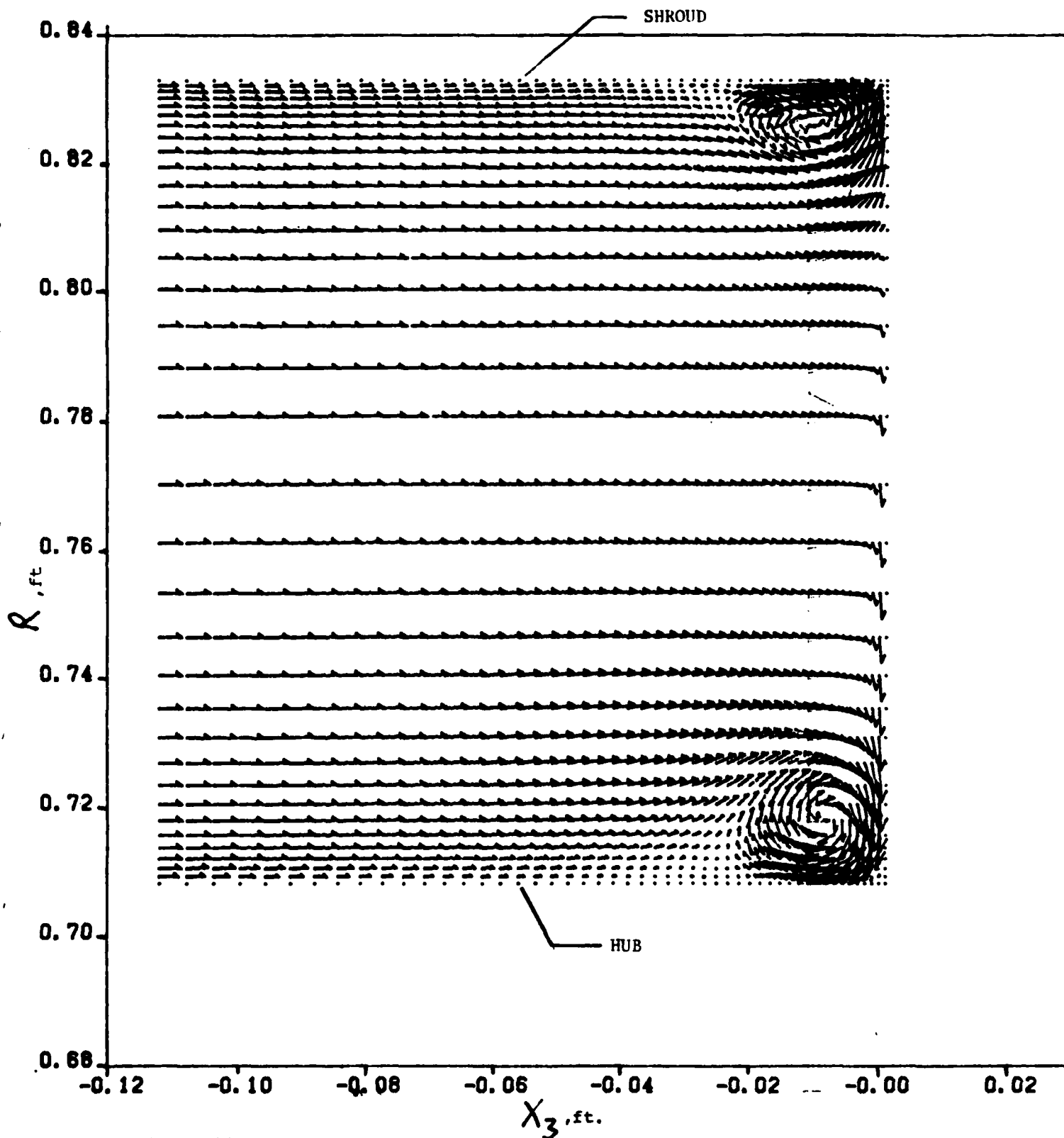
Figure 26. Velocity vector plot of the time-averaged meridional flow field at \alpha = -1.660508 radians; _____
