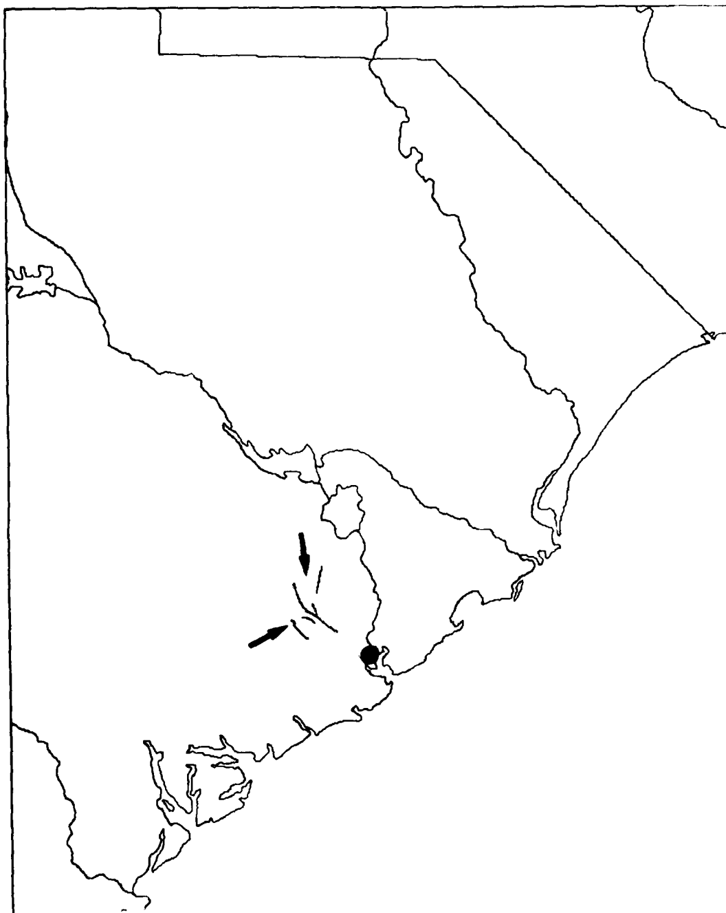
Figure 37. Seismic lines (arrows) shot by Virginia Tech in Charleston area.
