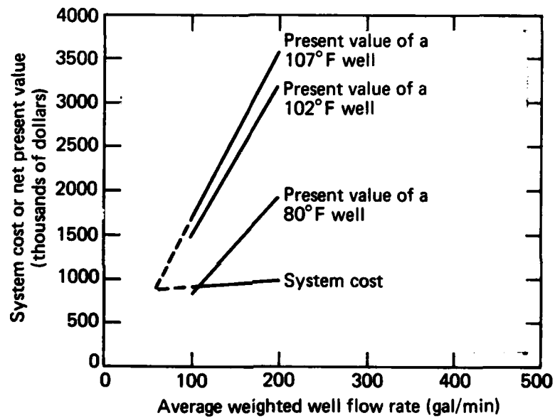
Figure 23. System cost and net present value as functions of average weighted well flow rate (Norfolk).
