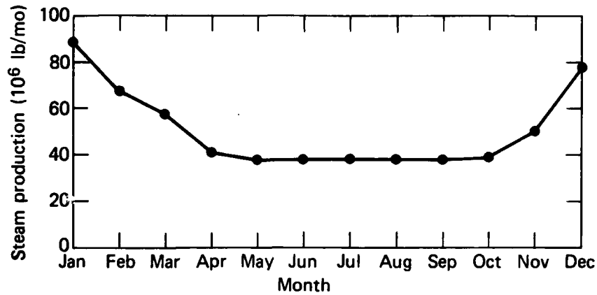
Figure 27. Jacksonville NARF monthly steam production--1981.
