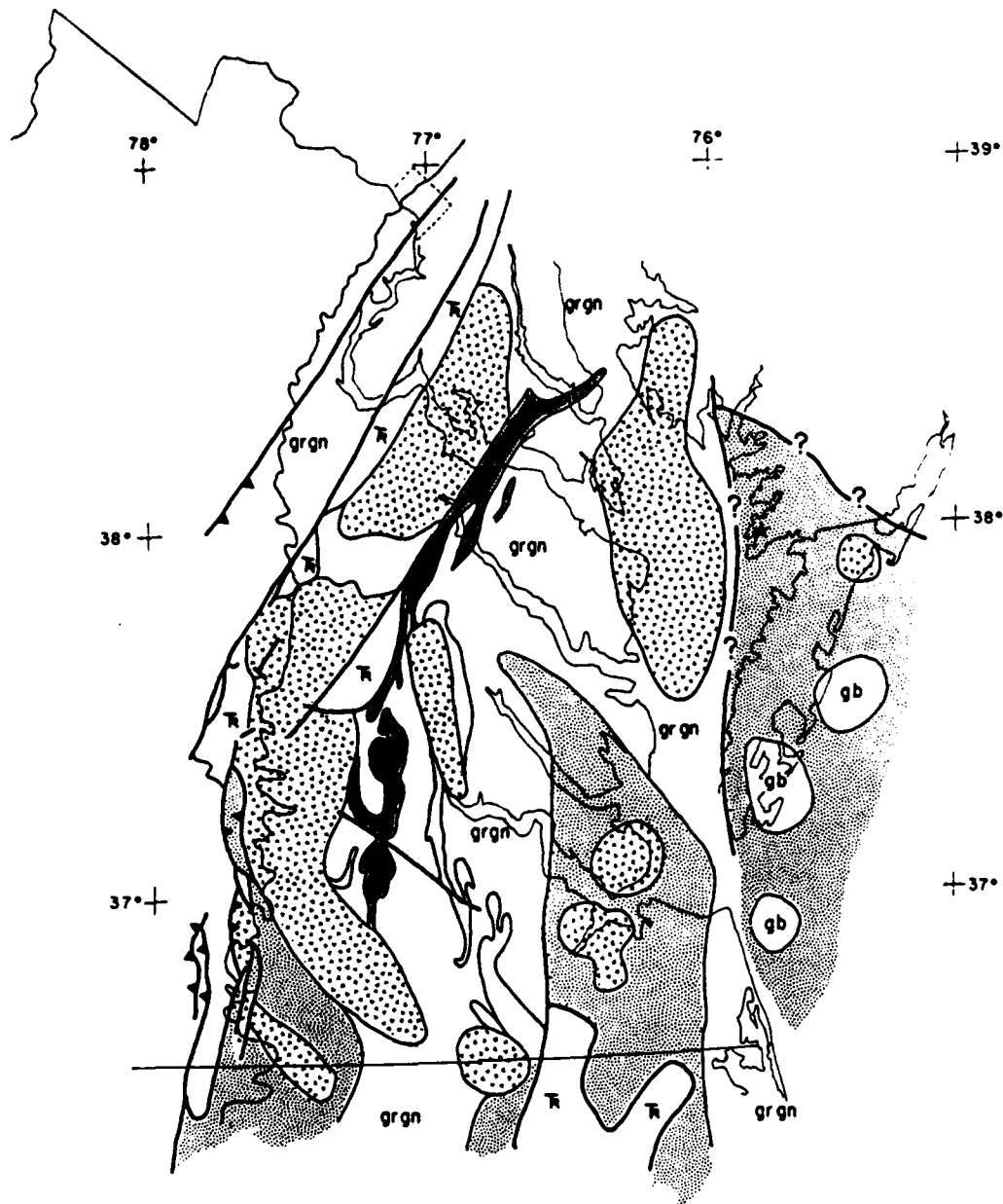
Figure 6. Generalized basement lithologies in eastern Virginia. gr=granitoid gneiss; v pattern = granite; fine stipple = low grade volcanics; dark cross line pattern = diorite or gabbro; gb=gabbro; Tr = Triassic/Jurassic ss. Interpretation by Glover and Costain from available basement samples, magnetic, and gravity data.
