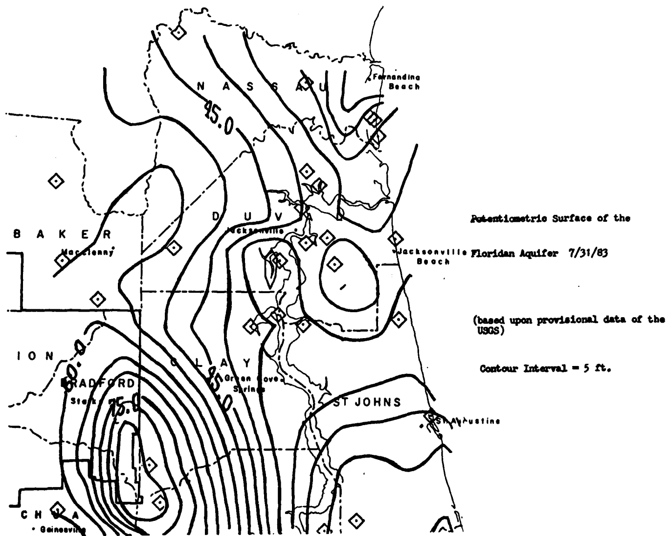
Figure 25. Potentiometric surface of the Floridan aquifer.
