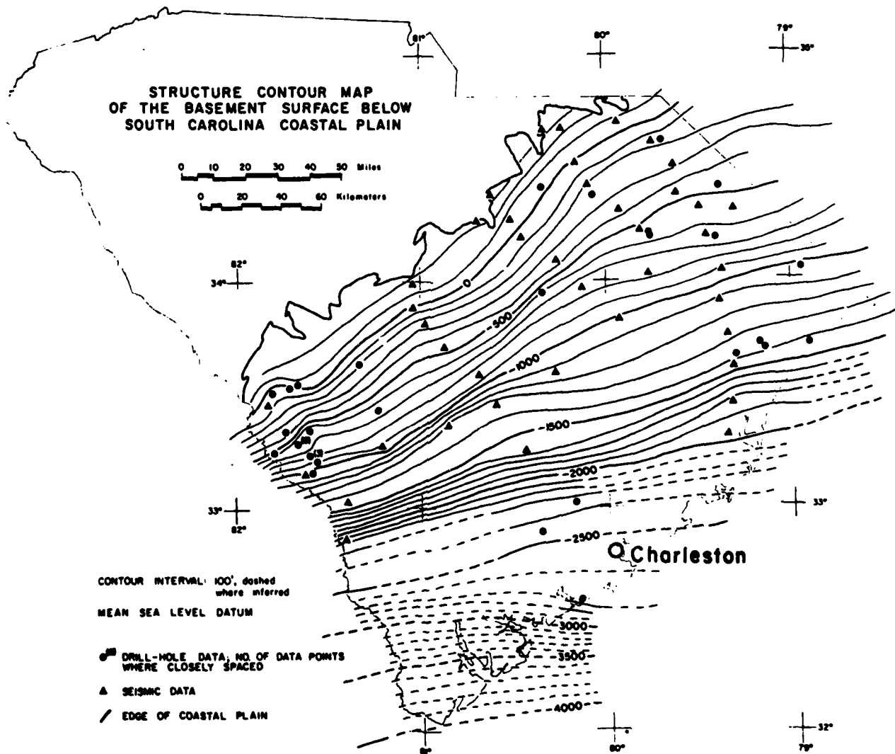
Figure 34. Structure contour map of the basement surface below the South Carolina Coastal Plain (Gleason, 1982).
