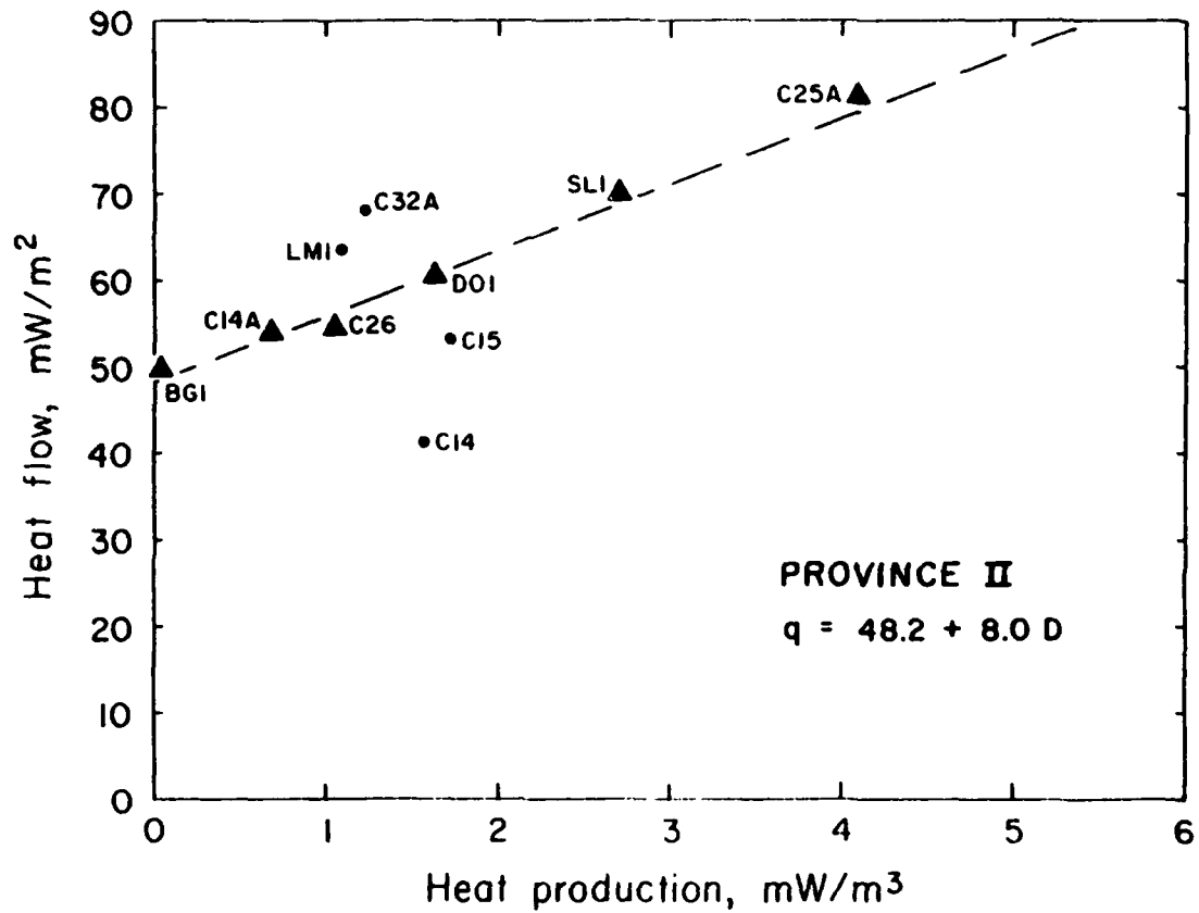
Figure 17. Linear relation between heat flow and heat generation for 'Province II' in the southeast United States (Costain and others, 1982a).
