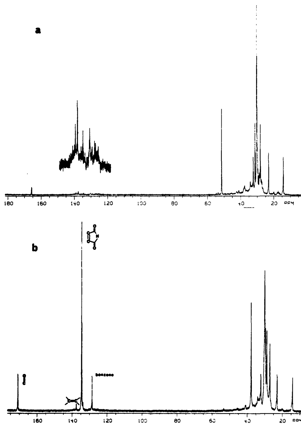
FIGURE 3. ^{13}\text{C} NMR (Acetone- d_6 ) of Dimer Diamine (a) and its Bismaleimide (b).
