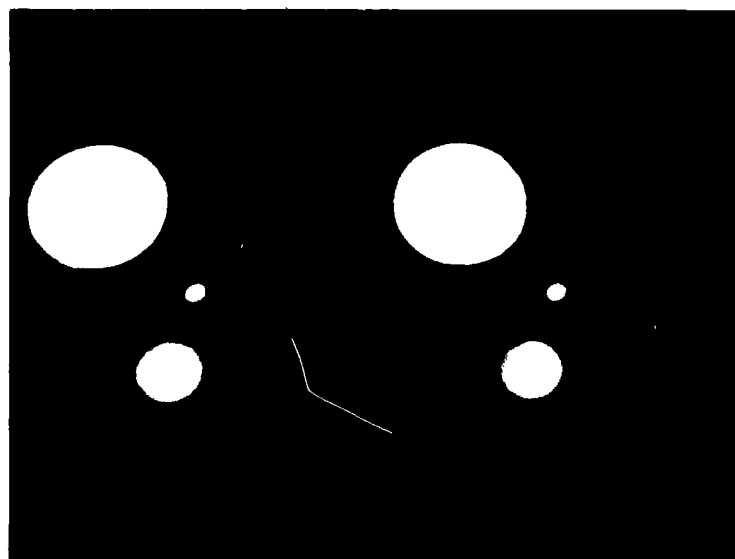
Figure 6 Reconstructed neutron tomograms showing effects of correction for scatter. Left: uncorrected, right: corrected for scatter
