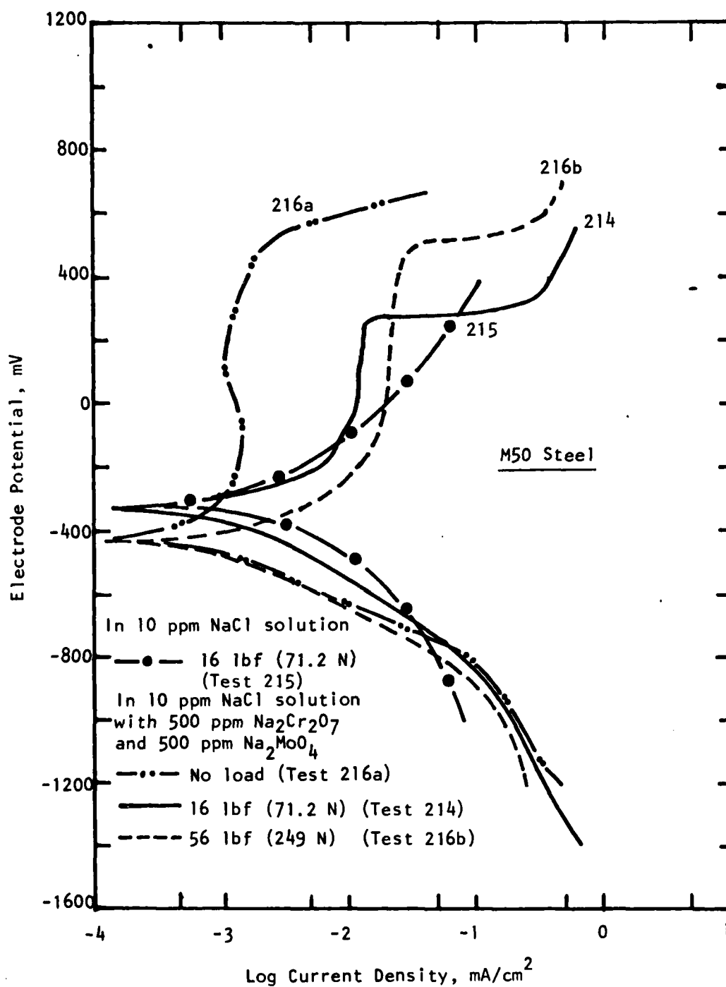
Figure 22. Polarization behavior of M50 steel in different electrolytes with oscillatory motion under various loads, 60° ( \pi/3 rad) amplitude, 1 cpm (17 mHz) (tests 214, 215, 216a, and 216b).
