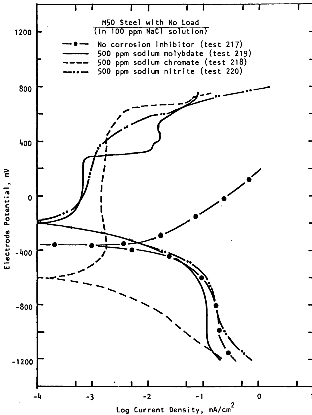
Figure 19. Effect of corrosion inhibitor on the polarization behavior of M50 steel under no-load conditions, 60° ( \pi/3 rad) amplitude, 1 cpm (17 mHz) (tests 217, 218, 219, and 220).
