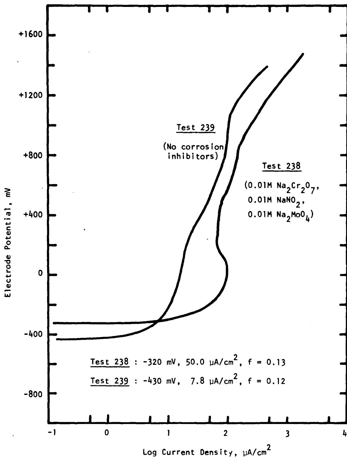
Figure 57. Effect of corrosion inhibitors on the polarization behavior of M50 steel in 100 ppm NaCl solution with 10% water-soluble oil under 56 lbf (249 N) at 10 cpm (170 mHz).
