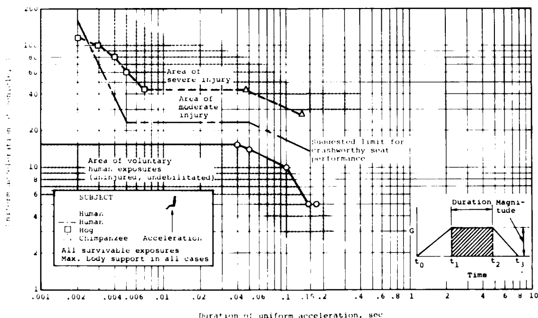
FIGURE 6.--Eiband Tolerance Curve for Vertical ( +G_z ) Accelerations
