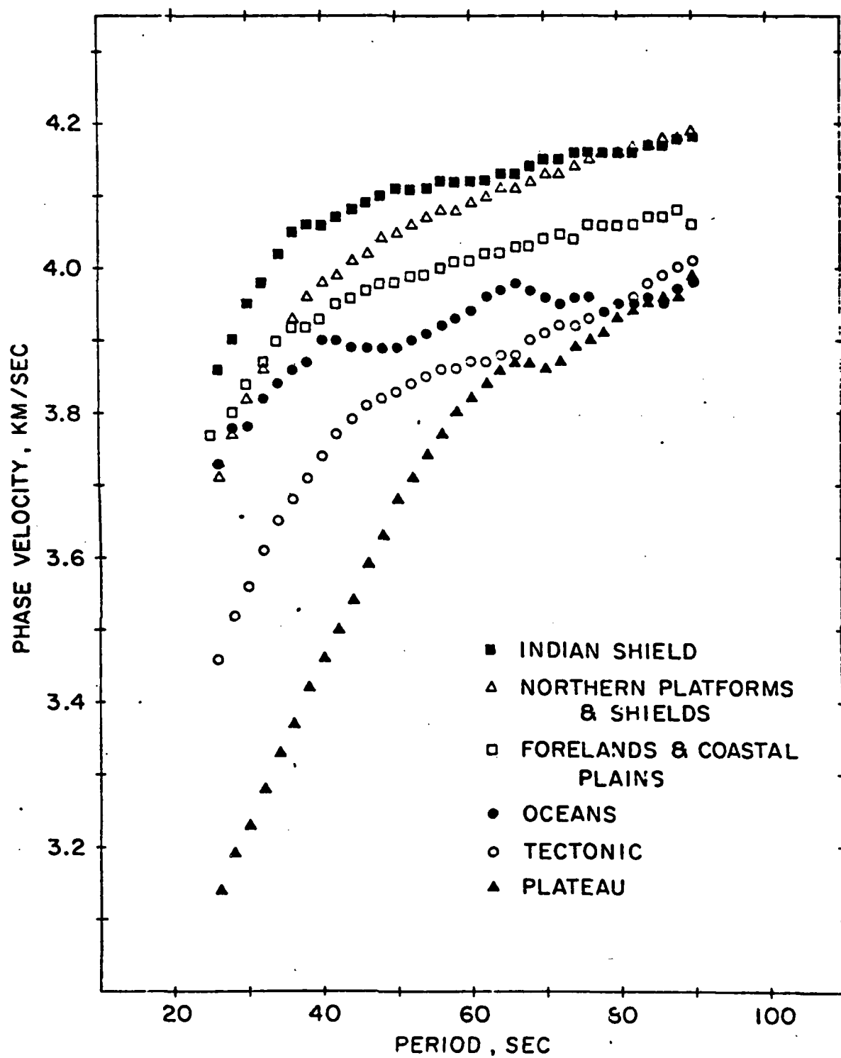
Fig. 5-2.3: Regionalized Rayleigh wave phase velocities.
