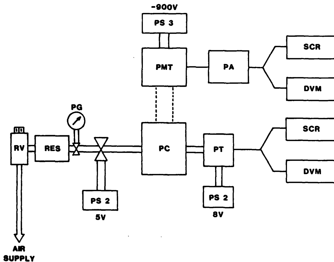
FIGURE 11: EXPERIMENTAL SETUP
