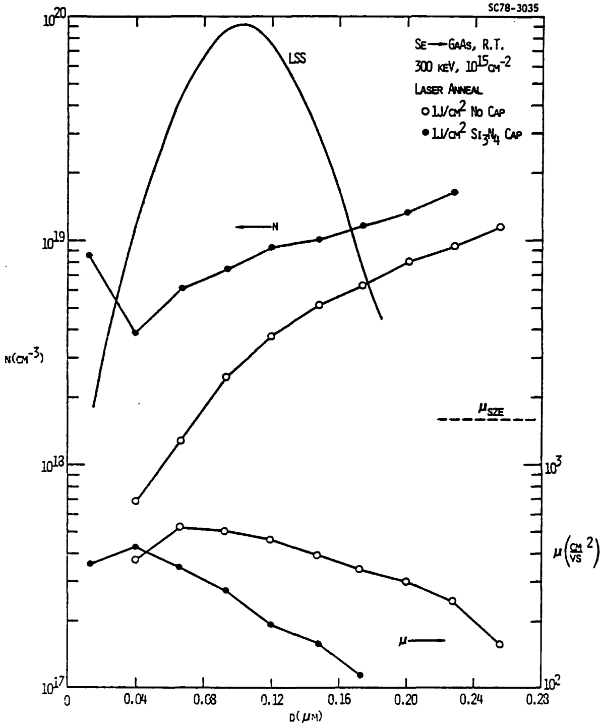
Fig. 2 Depth profiles of the electron concentration (N) and of the electron mobility ( \mu ) measured in the two laser annealed samples (Table I), one annealed with and the other without a Si 3 N 4 encapsulant. The incident energy densities employed were the same in the two samples.
