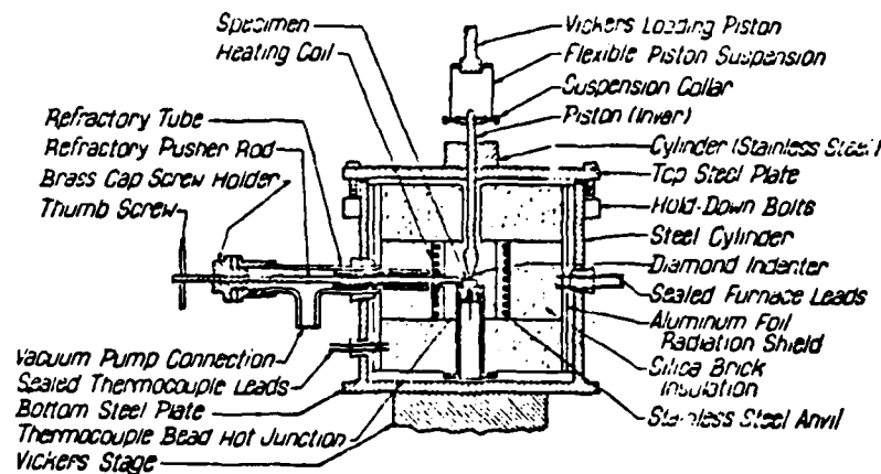
Fig 1a Design of Hot Hardness Tester.
