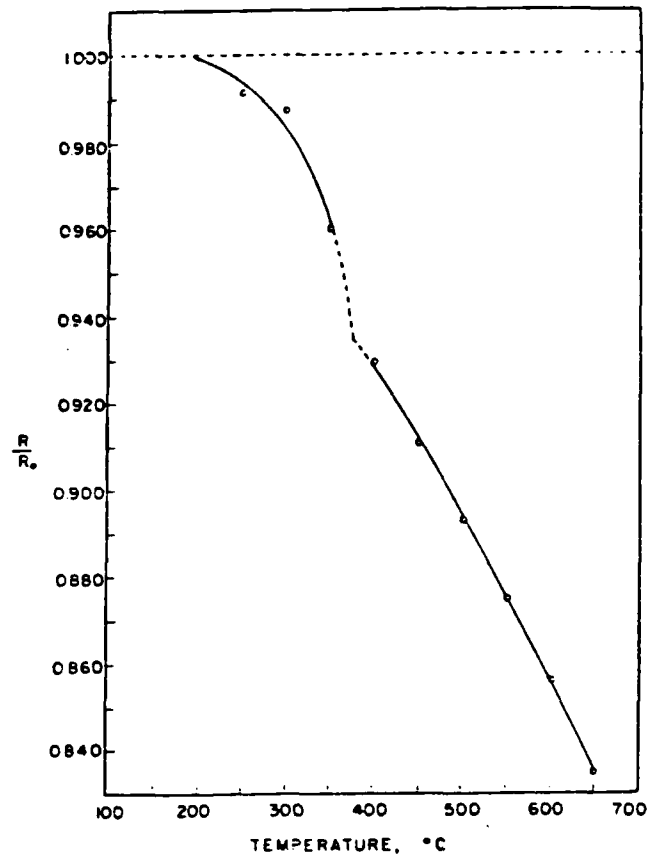
Fig. 2 -Isochronal plot of resistivity ratio vs temperature; doped tungsten (time = 120 min).
