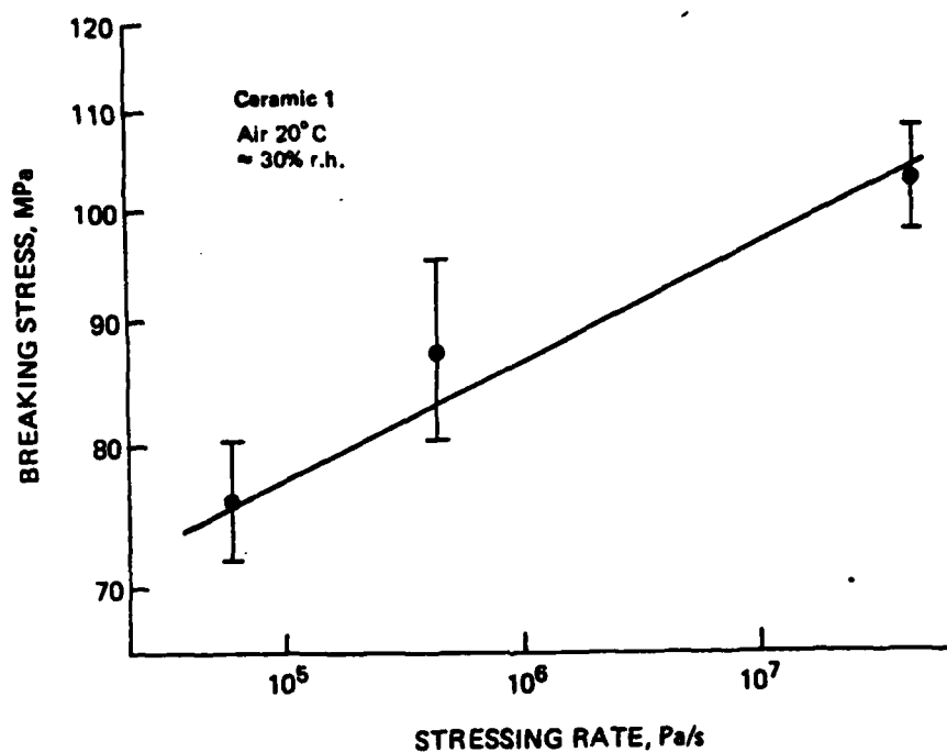
FIGURE 3 Strength-stressing rate curve for a typical capacitor material. The slope of the curve equals (n+1)^{-1} .
