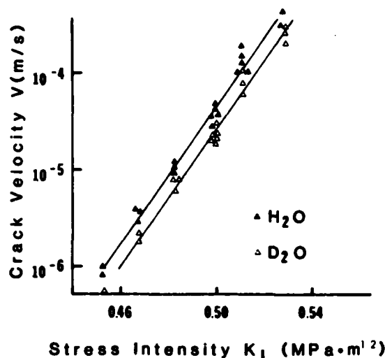
Fig. 5. Comparison of effects of H_2O and D_2O on slow crack growth in vitreous silica at room temperature.
