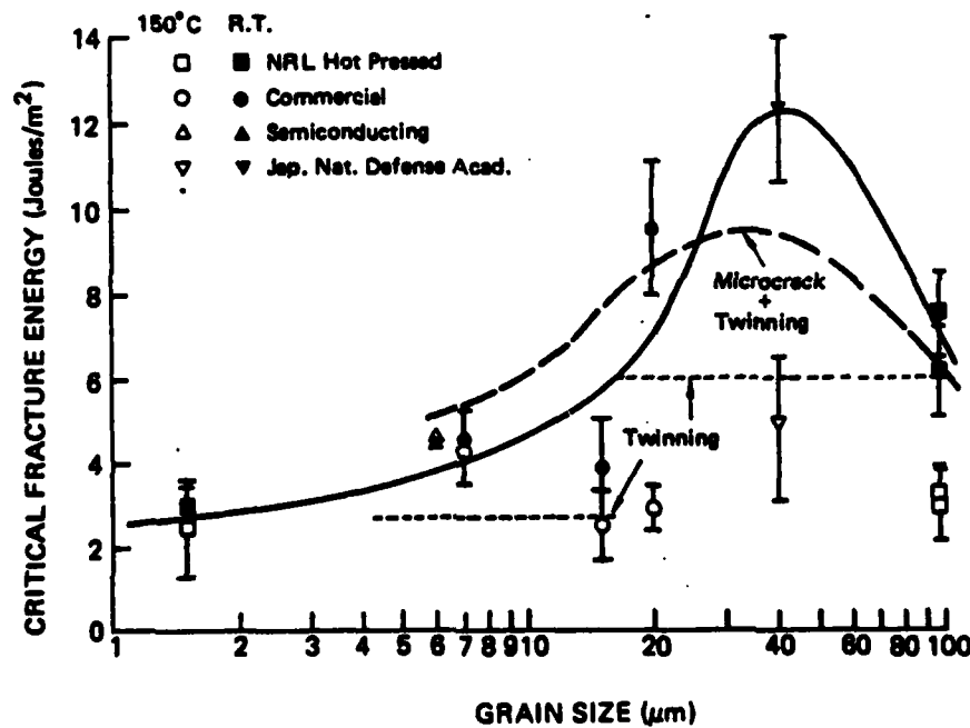
FIGURE 2 Fracture energy of \text{BaTiO}_3 as a function of grain size: — best fit to room temperature data; ---- contribution due to twinning, - - - combined effect of twinning and microcracking predicted by model of Rice and Freiman (1981).
