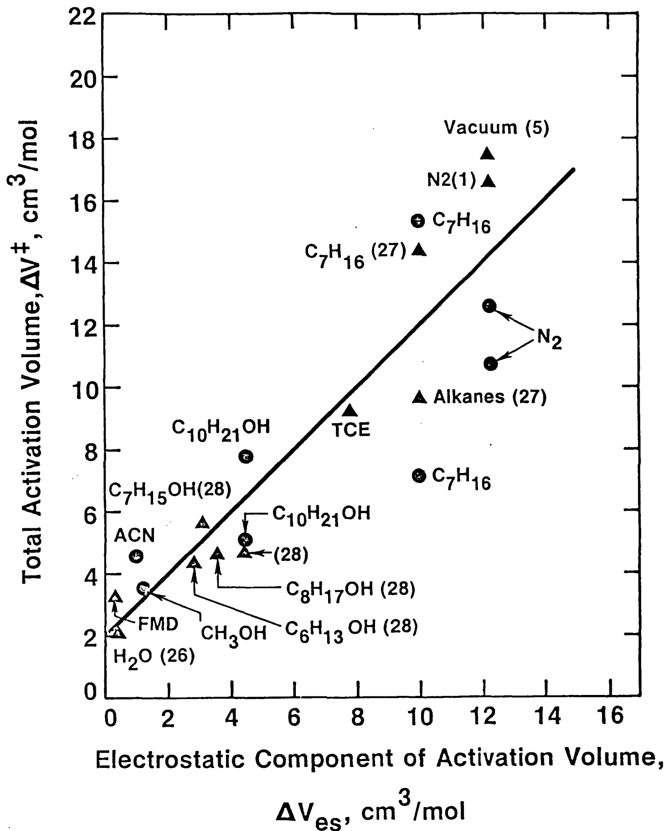
Figure 6. Activation volume, \Delta V_{\text{total}} , determined from the slope of the V-K I curve for soda-lime silica glass tested in environments whose dielectric constant varies from 1 (vacuum) to 78 (H 2 O plotted against the \Delta V_{\text{es}} calculated from Equation 8. (After Wiederhorn et al. [1982]).
