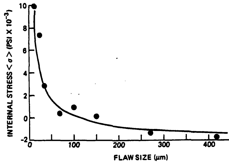
FIGURE 1 Effective internal tensile stress in fine-grained \text{BaTiO}_3 , determined from measurements of flaw sizes, fracture stress and critical fracture energy, as a function of measured-flow size.
