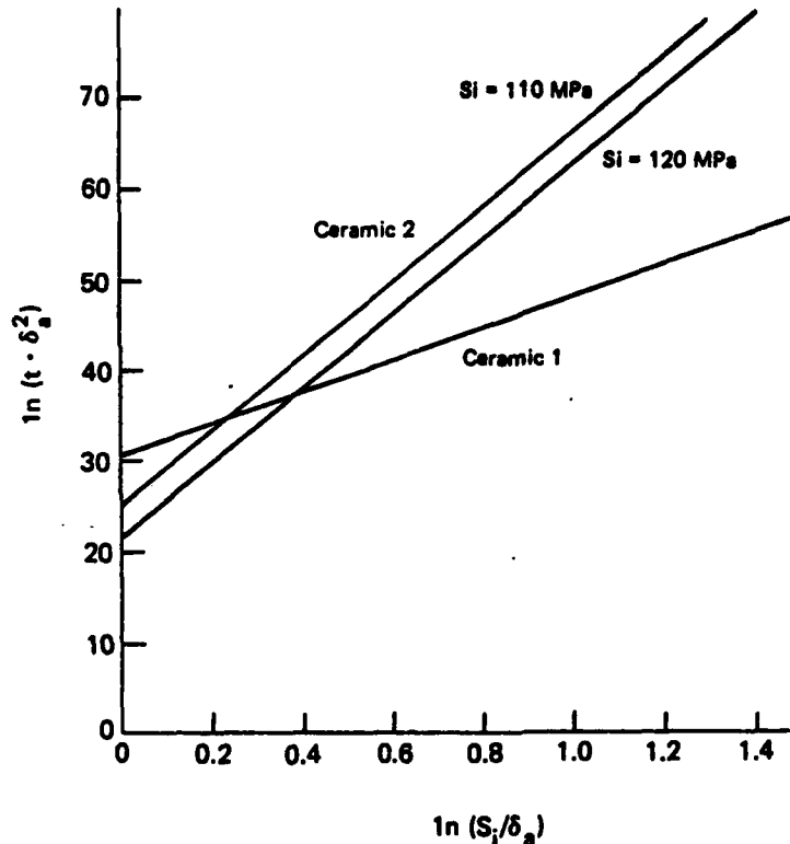
FIGURE 5 Comparison of failure time predictions for two capacitor materials. Ceramic 1: n = 19.5 and \ln B = 30.95 . Ceramic 2: n = 42.2 and \ln B \approx 27.0 .
