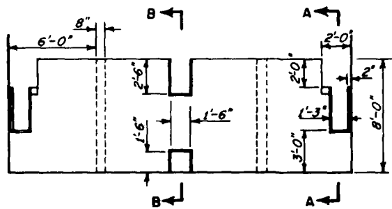
DOWNSTREAM ELEVATION
