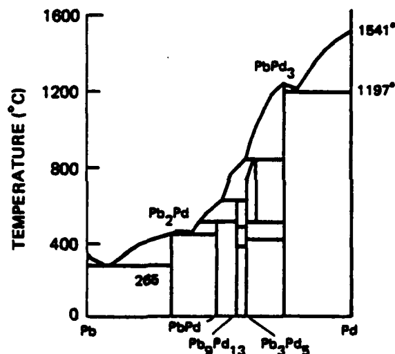
FIGURE 23 Palladium-lead phase diagram.
