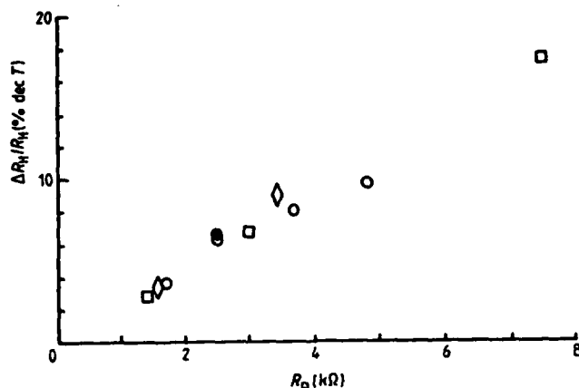
Figure 3. The percentage change in the Hall constant, per decade change in temperature, plotted against resistivity (sheet resistance) R_{\square} for three devices. The threshold voltages and mobilities \mu of these devices were adjusted by ion implantation. The values of \mu ( \text{m}^2 \text{V}^{-1} \text{s}^{-1} ) and magnetic field B (T) were as follows: \square B = 0.1 T, \mu = 0.39 ; \circ B = 0.1 T, \mu = 0.29 . \bullet was the same device as \circ but B = 0.61 T; \diamond B = 0.1 T, \mu = 0.23 . As seen the results \circ and \bullet are identical for the same value of R_{\square} and are independent of magnetic field.
