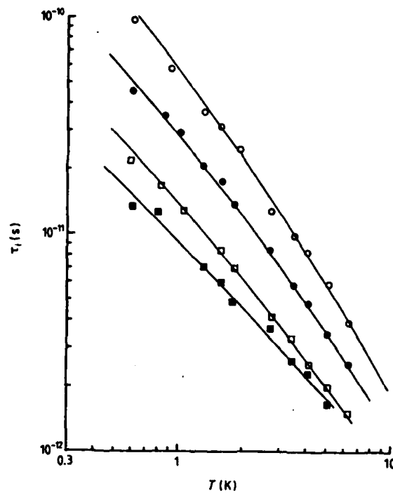
Figure 3. The inelastic scattering time \tau_i , in seconds, is plotted against temperature for a JH1/15 device. The lines are fitted curves 1/\tau_i = A_1T + A_2T^2 ; further details are given in table 2.
