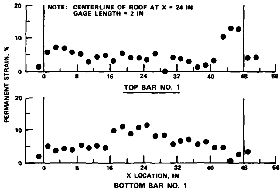
PERMANENT STRAIN OF REBAR FOR DS3
