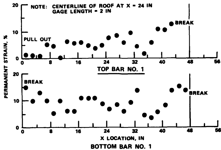
PERMANENT STRAIN OF REBAR FOR DS5
