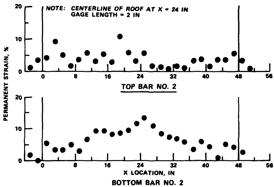
Figure 4-13. Permanent Strain of Rebar for DS3.
