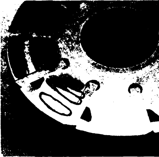
Left - Closeup up of rotor top; the dark and bright areas circled are bronze buildup off of the wear plates.
