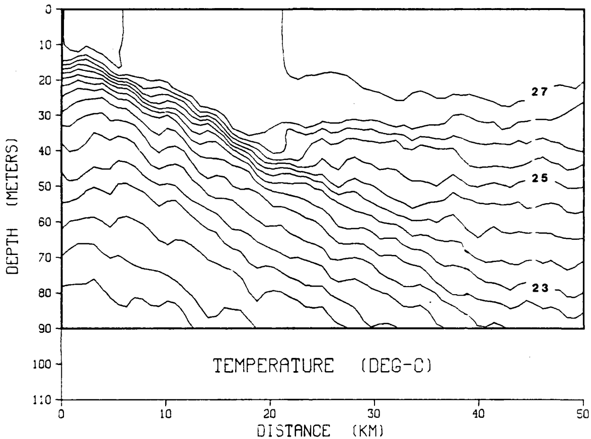
Fig. 2. Temperature contours in 0.5^{\circ} C increments along a northward track of the USNS Hayes on 20 July 1981 as it crossed the Subtropical Front. (From Trump et al, 1984.)
