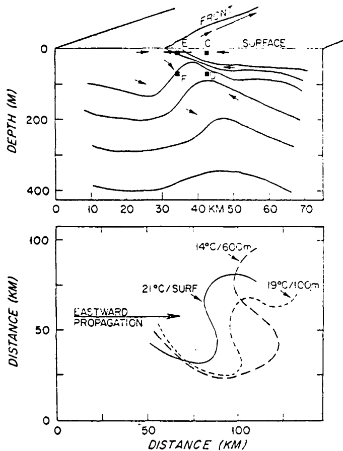
Fig. 1. Upper: Vertical temperature distribution across front on 15 March 1977 (contour interval is 1^{\circ}\text{C} ). Superimposed schematically, are the positions of drogues relative to front and current direction during frontogenesis.
