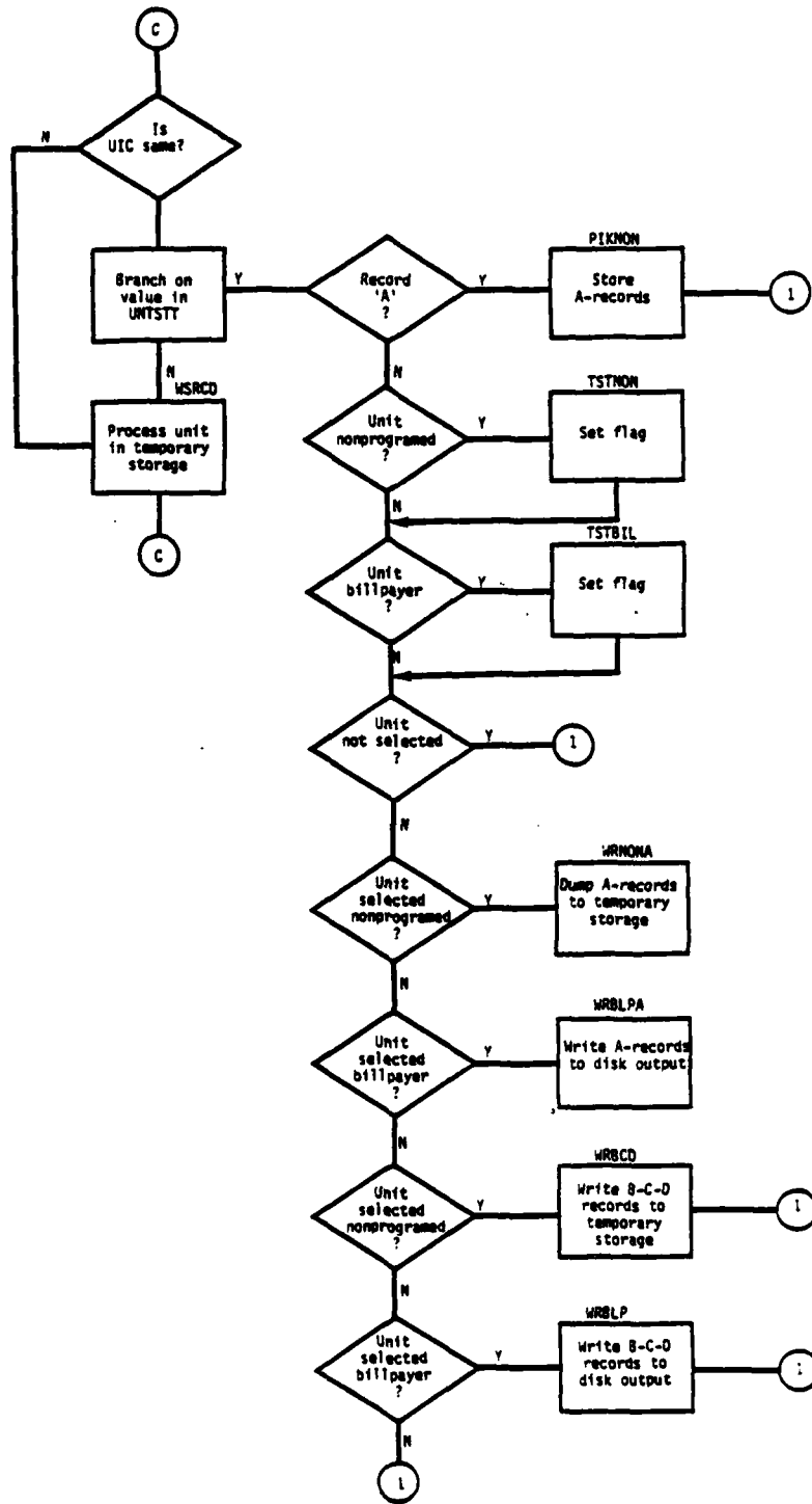
Figure 2-2. Tape Processor Flow Diagram (page 4 of 4 pages)
