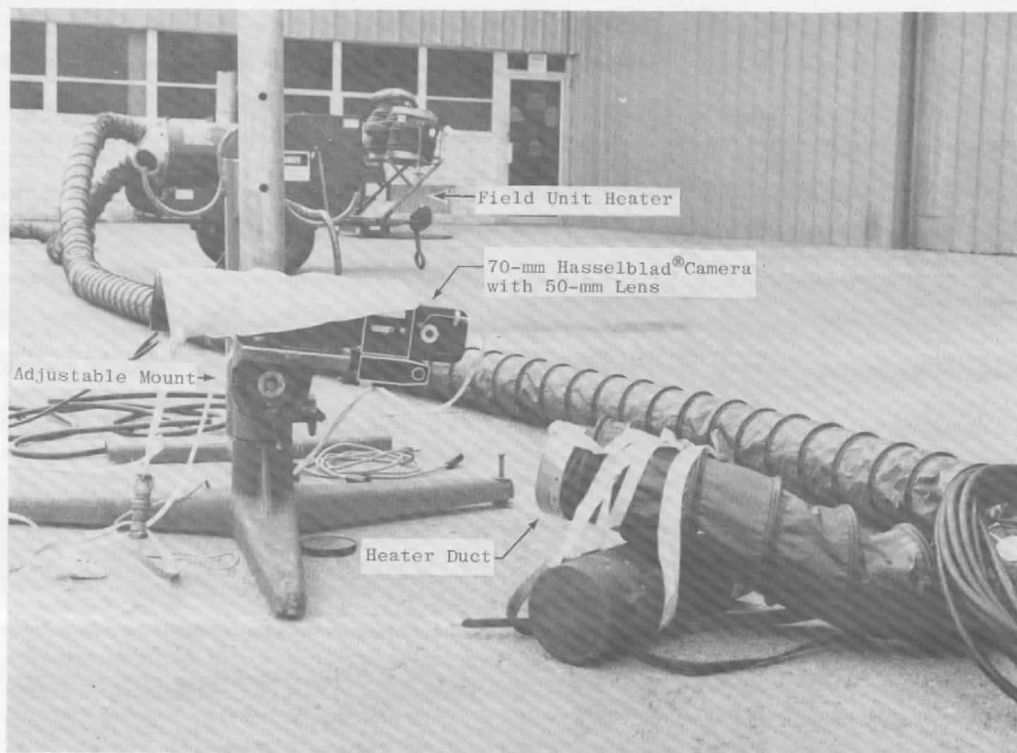
Figure 14. Camera test installation and heating system.
