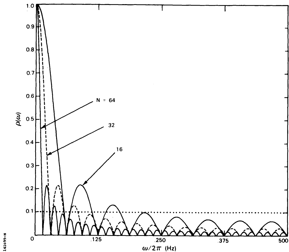
Fig. 1. \rho(\omega) vs \omega for N=16, 32 and 64 .
