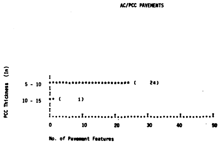
Figure 23. Histogram of AC/PCC Pavement Concrete Thickness in Inches.
