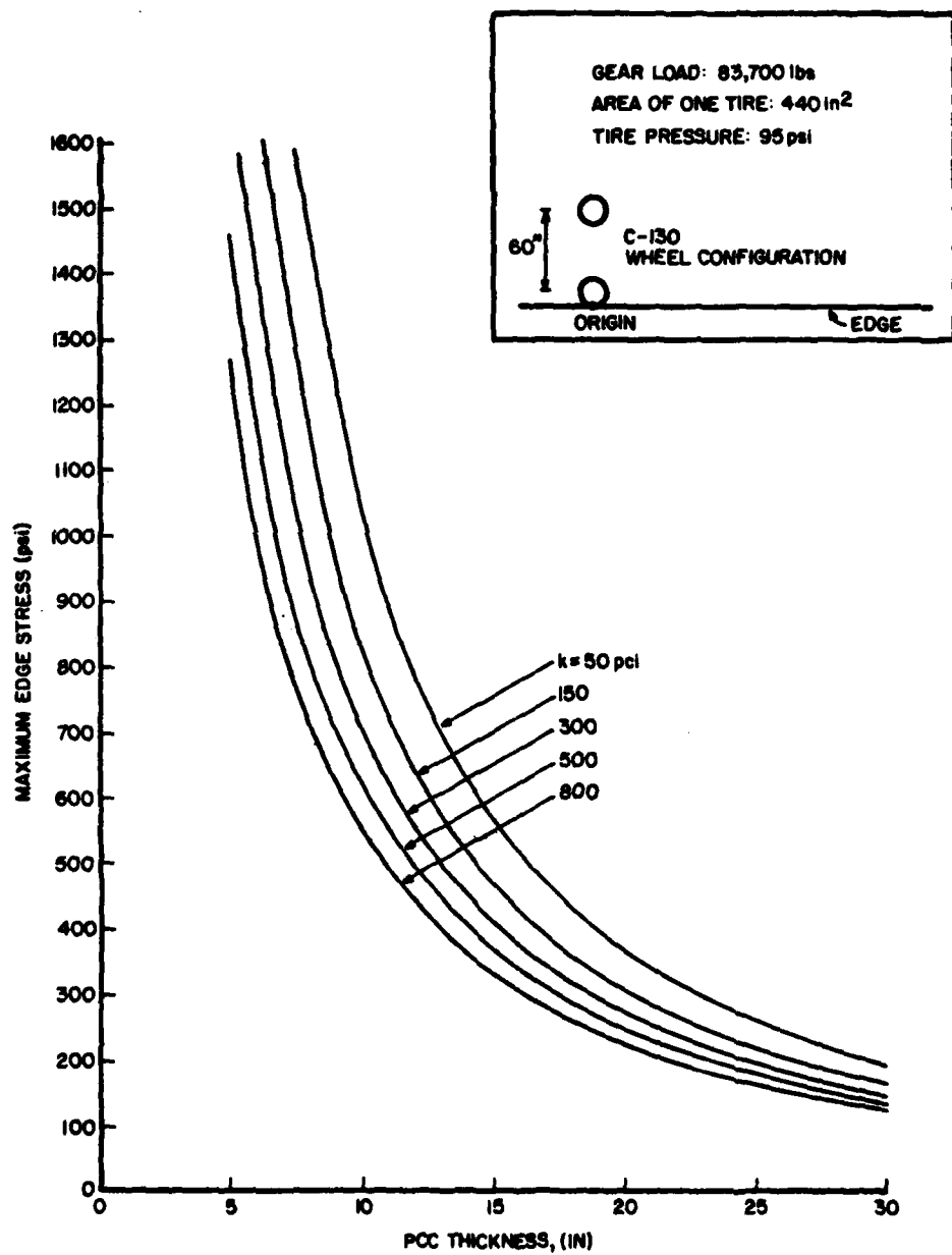
Figure B-15. Stress Chart for C-130.
