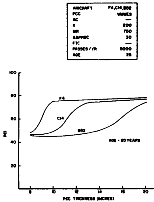
Figure 32. Effect of Aircraft Types on the PCI as a Function of PCC Thickness.
