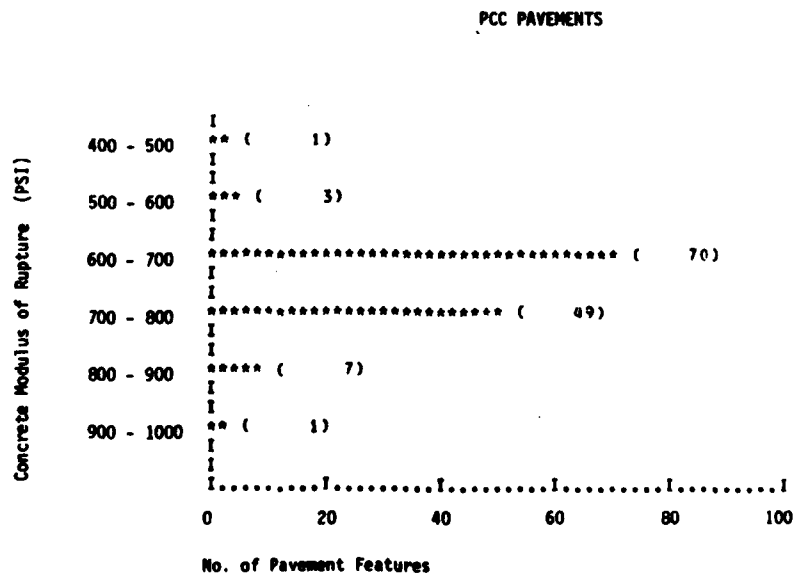
Figure 5. Histogram of Modulus of Rupture of Concrete in Pounds.
