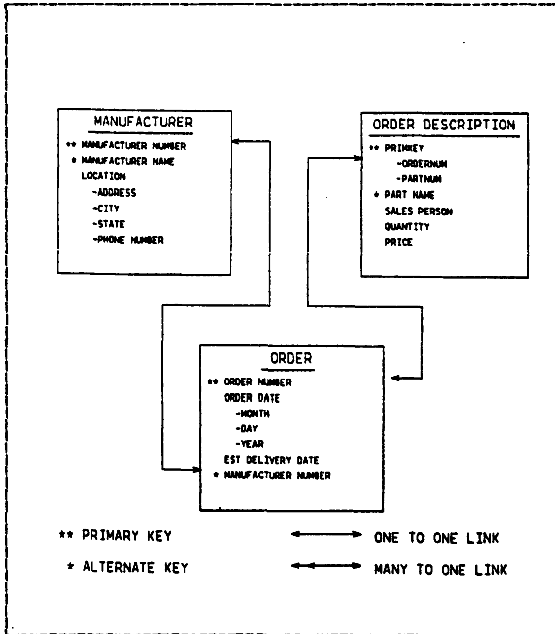
Figure 4.2 Manufacturer File.
