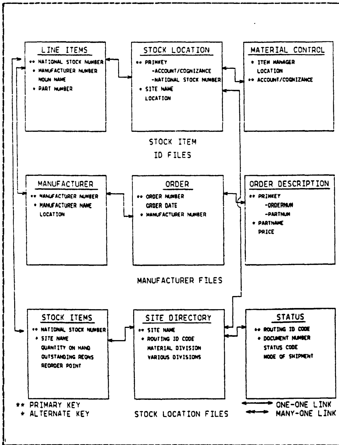
Figure 4.4 SPLICE Directory.
