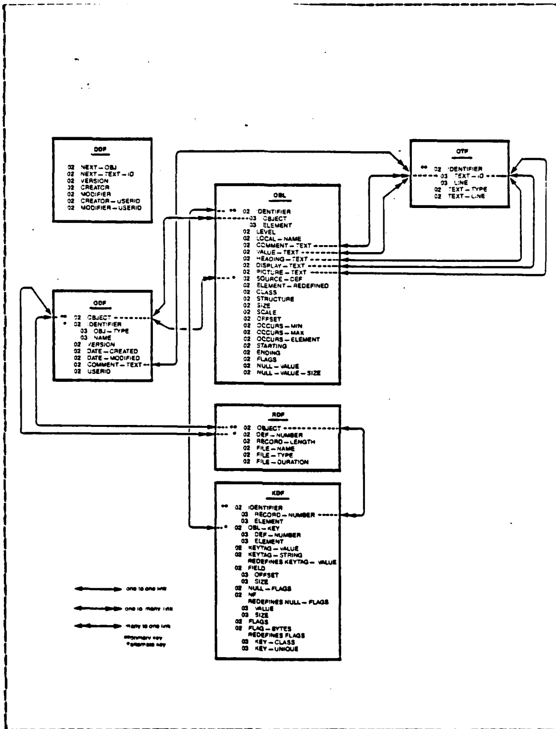
Figure 3.8 Dictionary Structure.
