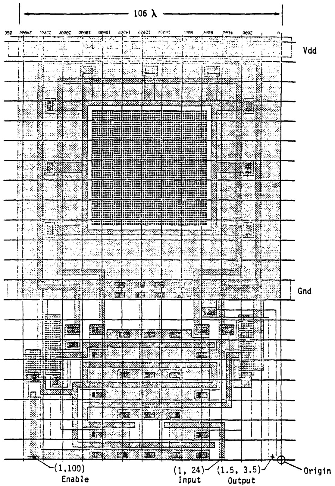
Figure 8 - Padtristate (4), rotated 90° CCW. 8 lambda grid. The "4" specifies now far the Gnd and Vdd tabs stick out.
