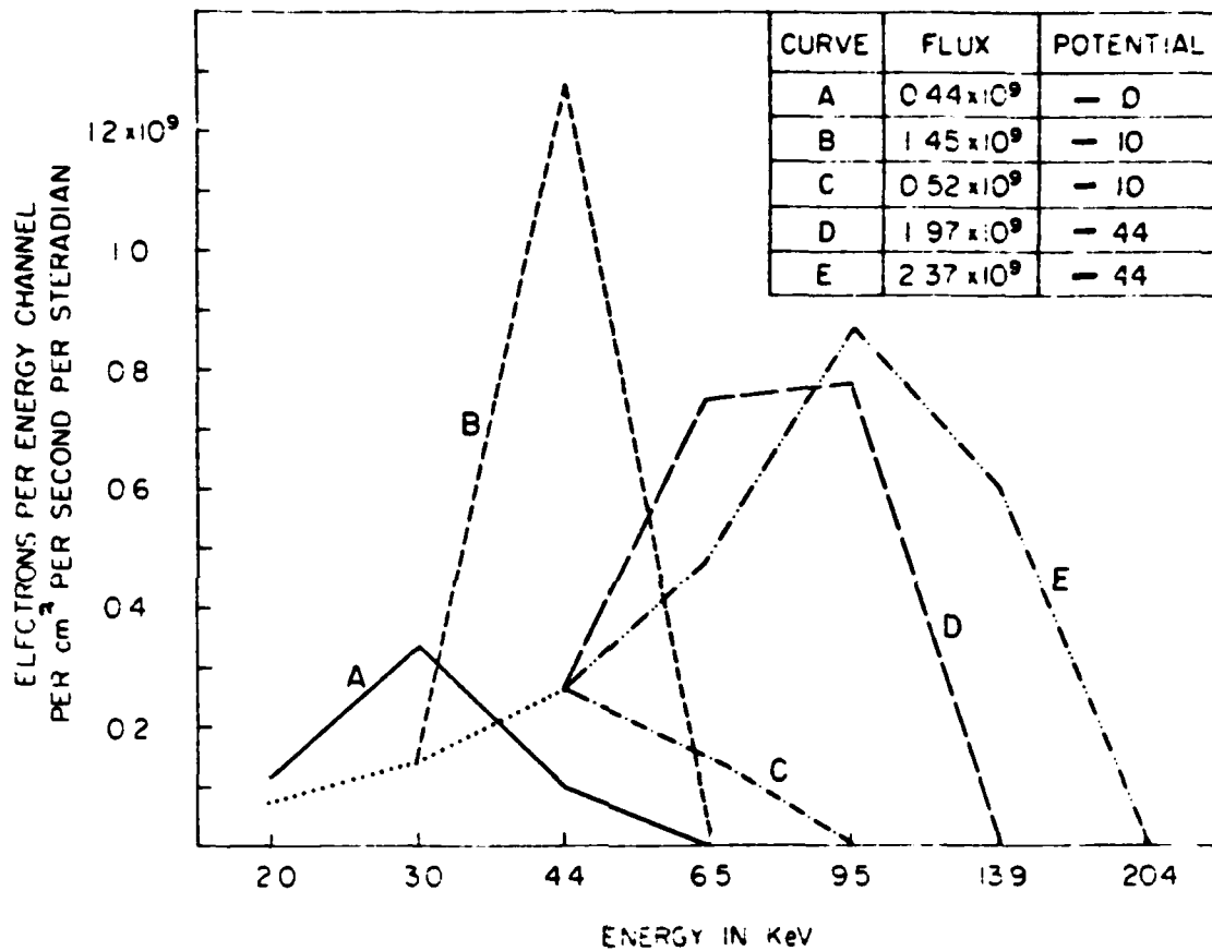
Figure 1: Five precipitating electron spectra. The flux associated with each spectra is listed in the upper right hand corner along with the corresponding spacecraft potential.
