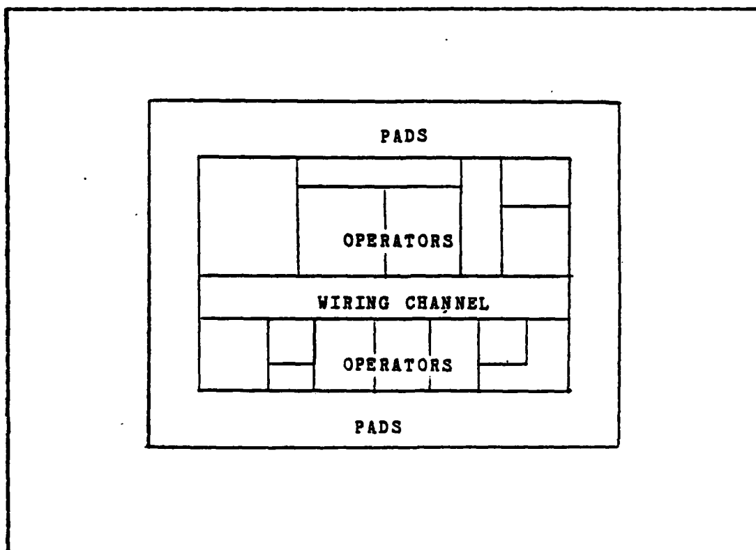
Figure 2.2 Typical floor plan produced by the F.I.R.S.T. Silicon Compiler.
