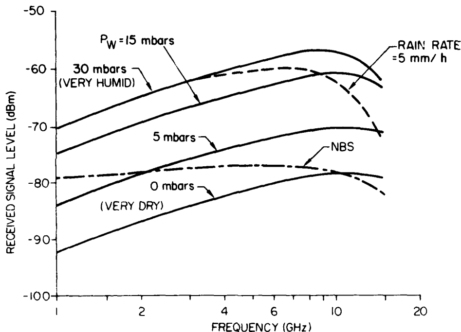
FIG. 20 Received signal level of troposcatter link compared to the National Bureau of Standards signal level. Based on 15-ft. antennas in a 100-km path. P_T = 100 W. (From Parl and Malaga, 1982.)
