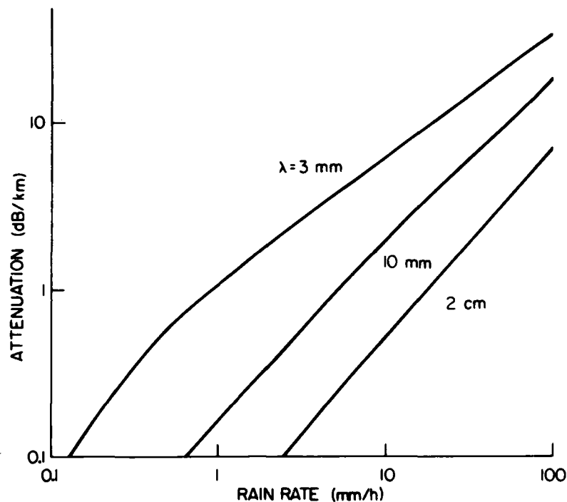
FIG. 10 Rain attenuation as a function of rain rate. (From Medhurst, 1965. © 1965 IEEE.)
