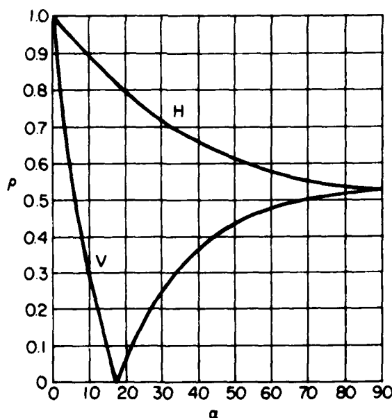
FIG. 4 Magnitude of reflection coefficient \rho for average land as a function of incidence angle \alpha ( \epsilon' = 10 , \sigma = 1.6 \times 10^{-3} S/m). (From "Airborne Radar" by Donald J. Povejsil, Robert S. Raven, and Peter Waterman. © 1961 by D. Van Nostrand Company, Inc. Reprinted by permission of Wadsworth Publishing Company, Belmont, California 94002.)
