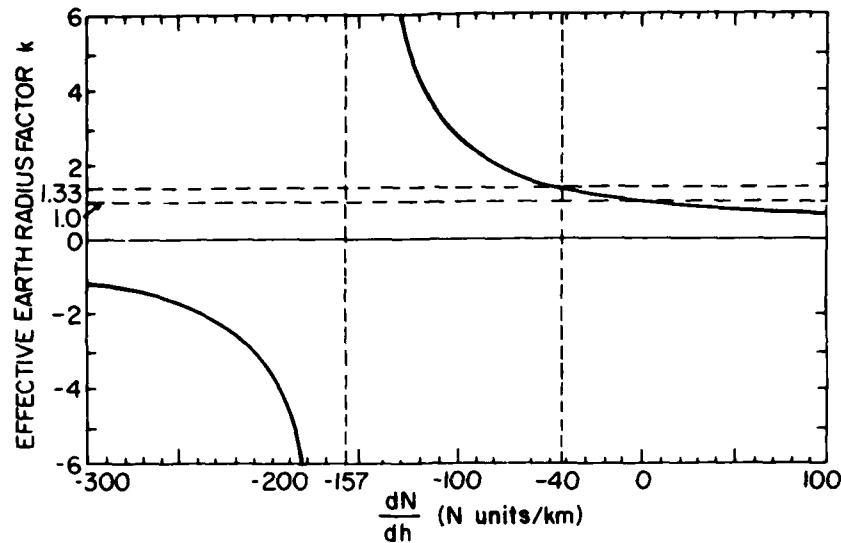
FIG. 2 Effective earth radius factor as a function of refractive index gradient dN/dh : ducting region, dN/dh < -157 N units/km, K < 0 ; supperrefraction region, -157 N units/km < dN/dh < -40 N units/km, 0 < K < \frac{4}{3} ; subrefraction region, -40 N units/km < dN/dh , \frac{4}{3} < K < 0 . (From Hall, 1979. © Peter Peregrinus Ltd.)
