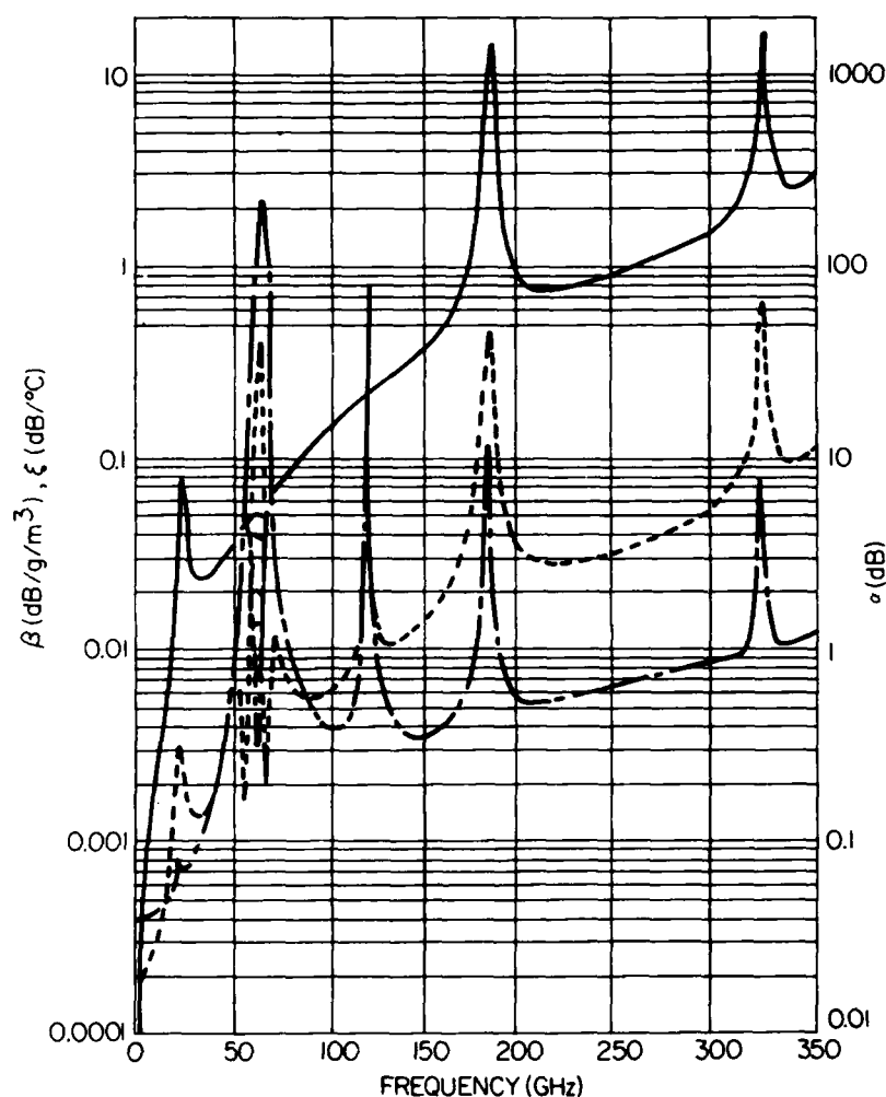
FIG. 15 Coefficients for computing zenith attenuation. Zenith attenuation \tau_{90^\circ} = \alpha + \beta\rho_0 - \xi T_0 (dB), with \rho_0 in grams per cubic meter and T_0 in degrees Celsius: — — —, \alpha coefficient; —, \beta coefficient; - - -, \xi coefficient. (From CCIR, 1982b).
