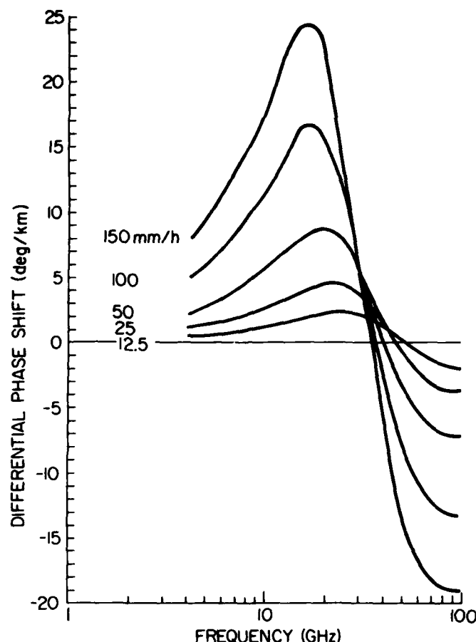
FIG. 12 Rain-induced differential phase shift. (From Hogg and Chu, 1975. © 1975 IEEE.)
