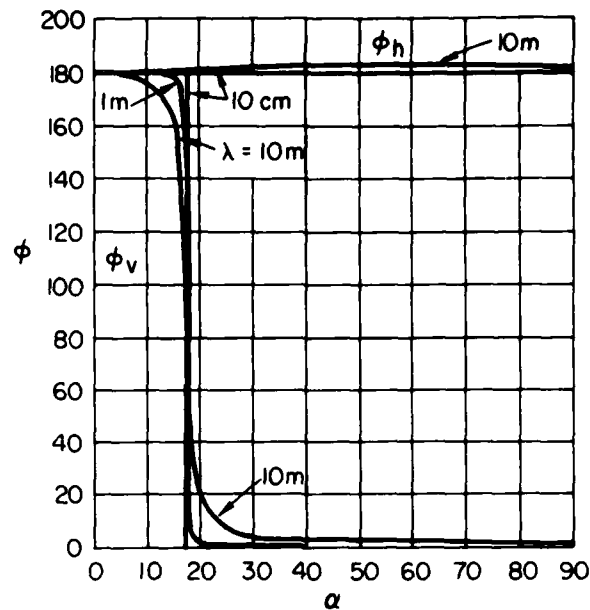
FIG. 5 Phase \phi of reflection coefficient for average land as a function of incidence angle \alpha ( \epsilon' = 10 , \sigma = 1.6 \times 10^{-3} S/m). (From "Airborne Radar" by Donald J. Povejsil, Robert S. Raven, and Peter Waterman. © 1961 by D. Van Norstrand Company, Inc. Reprinted by permission of Wadsworth Publishing Company, Belmont, California 94002.)
