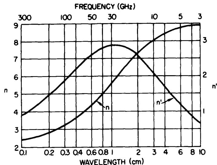
FIG. 7 Typical values of refractive indices of water at 20°C. (From Hogg and Chu, 1975. © 1975 IEEE.)
