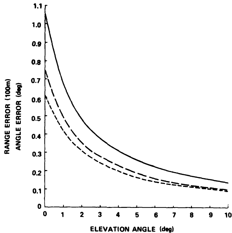
FIG. 1 Typical tropospheric refraction angle and range errors: —, range error; ---, angle error ( h = \infty ); -.-, angle error ( h = 90 km). CRPL reference atmosphere, 1958. (From Altshuler and Mano, 1982. Reproduced by permission of the U.S. Dept. of Commerce, National Technical Information Service, Springfield, Virginia 22161.)
