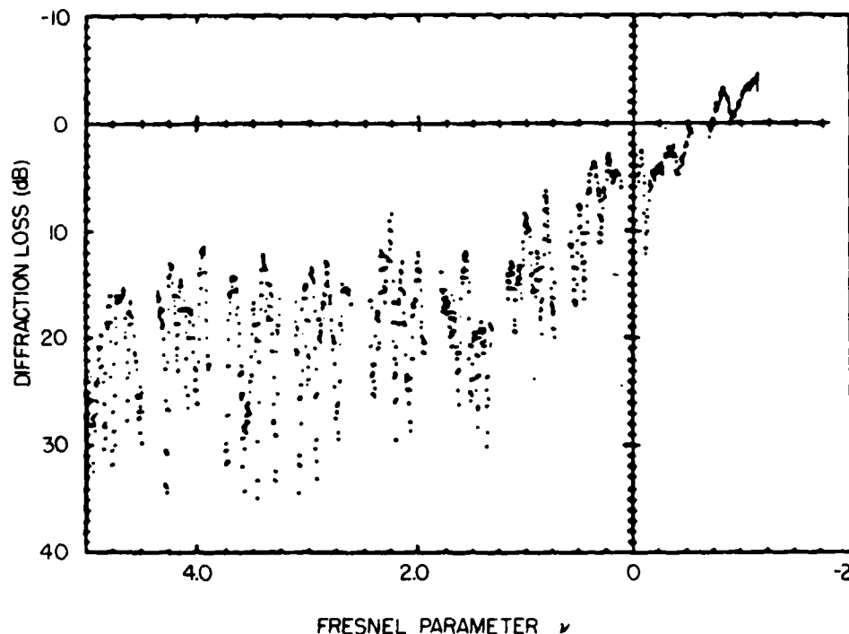
FIG. 21 Diffraction loss measured on a cluttered path with multiple diffraction. (From Haakinson et al. , 1980. © Reproduced by permission of the U.S. Dept. of Commerce, National Technical Information Service, Springfield, Virginia 22161.)
