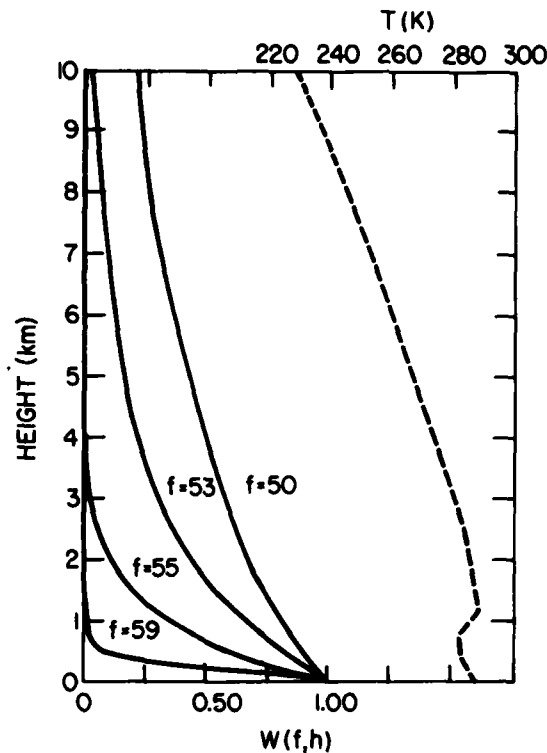
FIG. 23 Weighting functions for upward-directed temperature sensors (clear sky). (From Miner et al. , 1972. © American Geophysical Union.)
