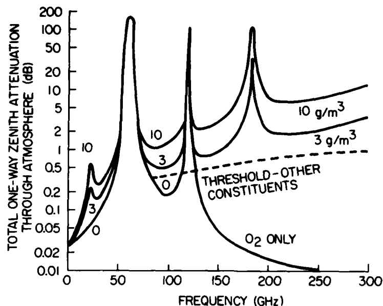
FIG. 16 Total zenith attenuation through atmosphere as a function of frequency. (From Smith, 1982. © American Geophysical Union.)
