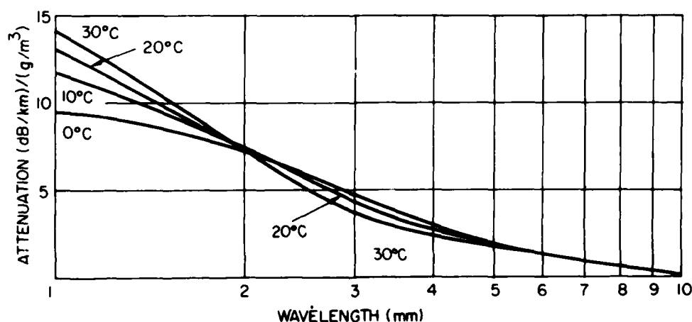
FIG. 13 Attenuation of cloud and fog as a function of wavelength.
