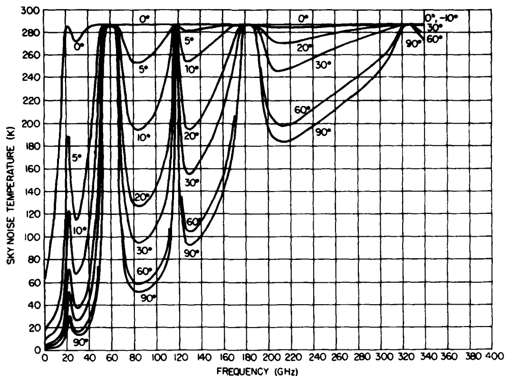
FIG. 17 Sky noise temperature as a function of frequency for a water vapor density of 7.5 \text{ g/m}^3 . (From CCIR, 1982).
