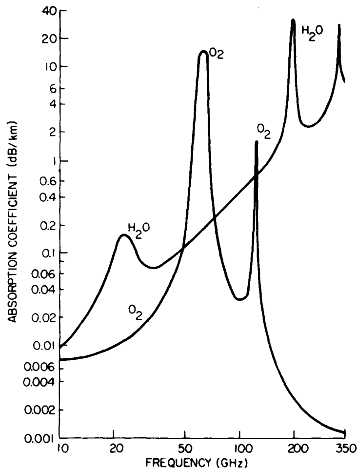
FIG. 3 Absorption coefficients for water vapor and oxygen. P = 1 atm, T = 20^\circ\text{C} , P_w = 7.5 g/m 3 . (From Smith, 1982. © American Geophysical Union.)
