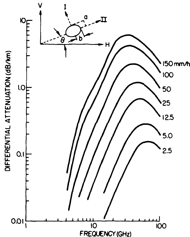
FIG. 11 Rain-induced differential attenuation. (From Hogg and Chu, 1975. © 1975 IEEE.)
