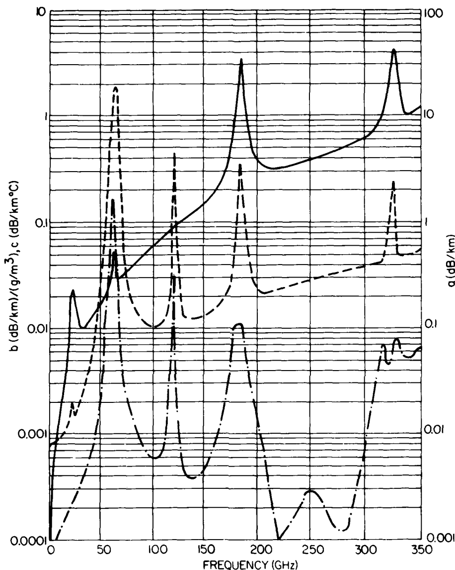
FIG. 14 Coefficients for computing specific attenuation. Specific attenuation A = a + b\rho_0 - cT_0 (dB/km), with \rho_0 in grams per cubic meter and T_0 in degrees Celsius: ---, a coefficient; —, b coefficient; — · —, c coefficient. (From CCIR, 1982a).
