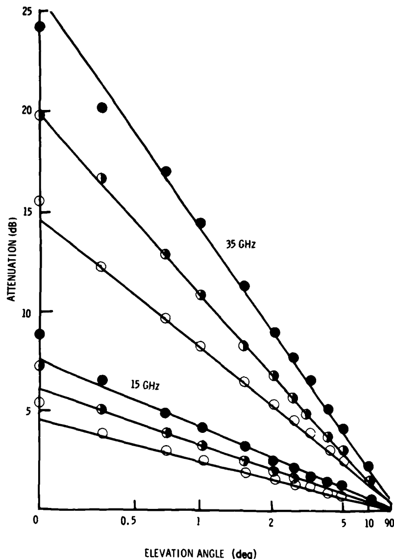
FIG. 18 Typical cloud attenuations as a function of elevation angle: ○, clear; ◐, mixed; ●, cloudy. (From Altshuler et al. , 1978. © Published by the American Geophysical Union.)
