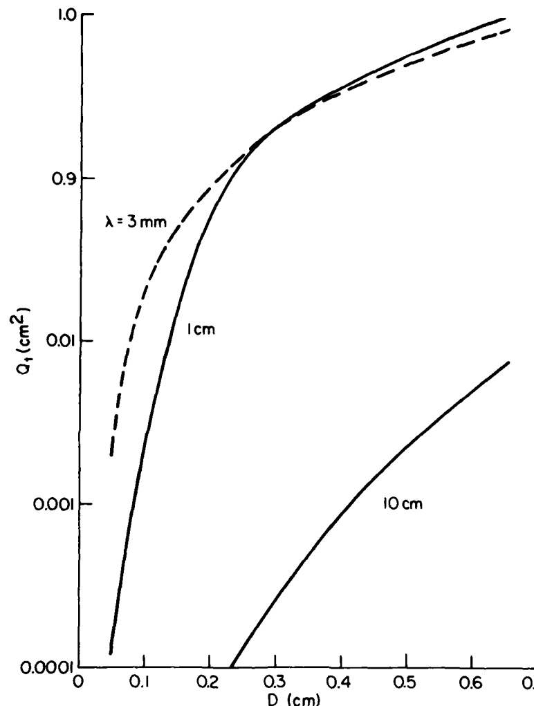
FIG. 8 Total cross section Q_t of a raindrop as a function of drop diameter D .
