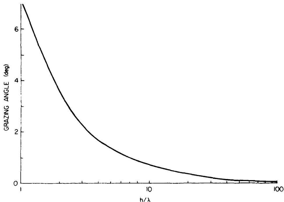
FIG. 6 Rayleigh roughness criterion.
