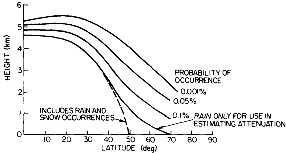
FIG. 19 0°C isotherm height for use in estimating the depth of the attenuating region on a slant path. (From Crane, 1980b. © 1980 IEEE.)
