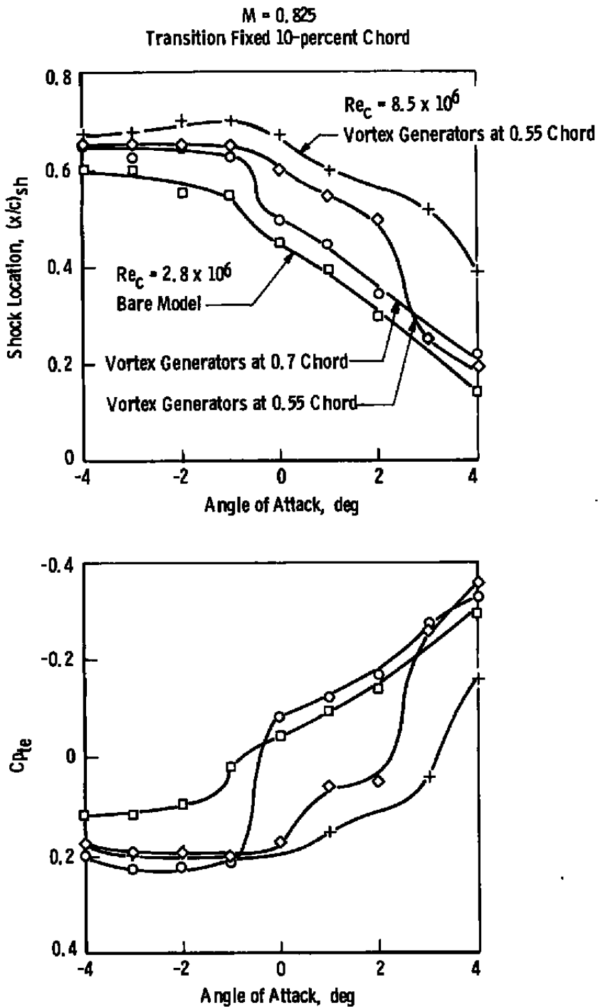
Figure 21. Effect of vortex generators on shock location and pressure recovery. From Cahill (Ref. 51)
