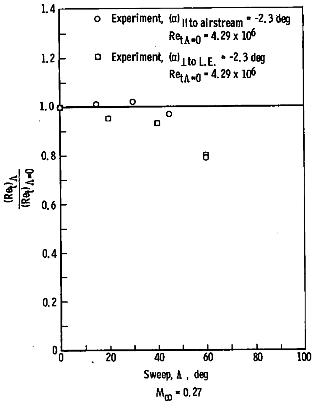
Figure 19. Variation of the normalized free-stream transition Reynolds number with sweep at subsonic Mach number. From Jillic and Hopkins (Ref. 49)
