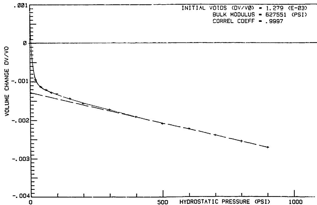
FIGURE 9. Hydrostatic Compression Properties of BLX-1. TEST FILE ID: D2/96 (C), SAMPLE ID: I-I-4A (06-28-83)
