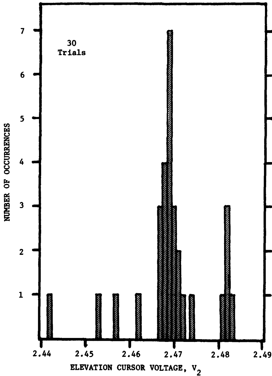
Figure 15. Histogram of cursor voltage for elevation beamsplitting trials on corner reflector No. 2.
