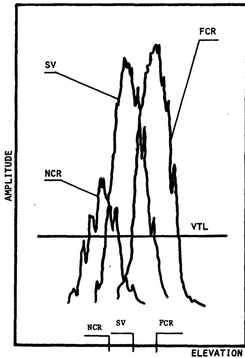
Figure 23. Radar elevation profiles: Run number A-3.
