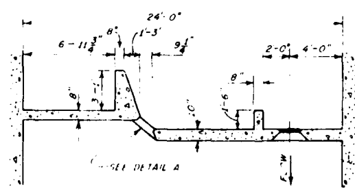
SECTION B-B
