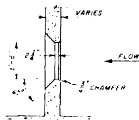
TYPICAL ORIFICE
