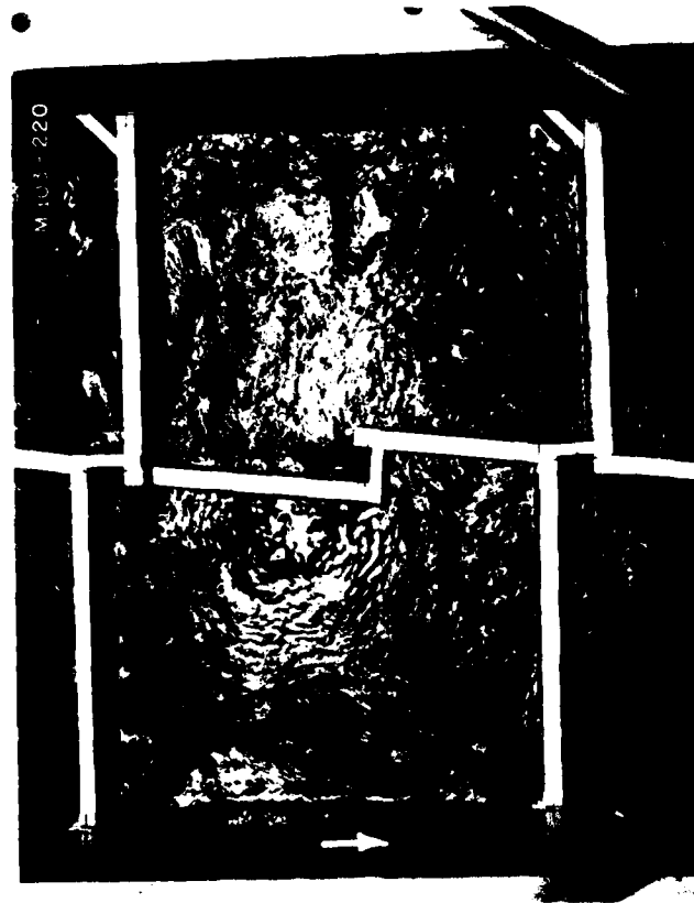
Pools 25 and 26
