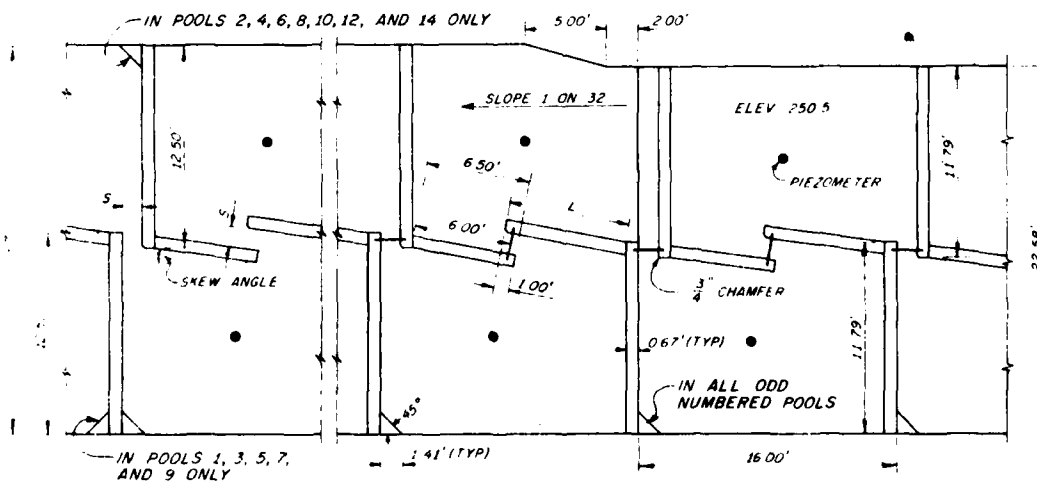
POOL DETAILS
