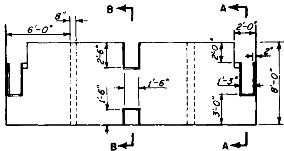
DOWNSTREAM ELEVATION
