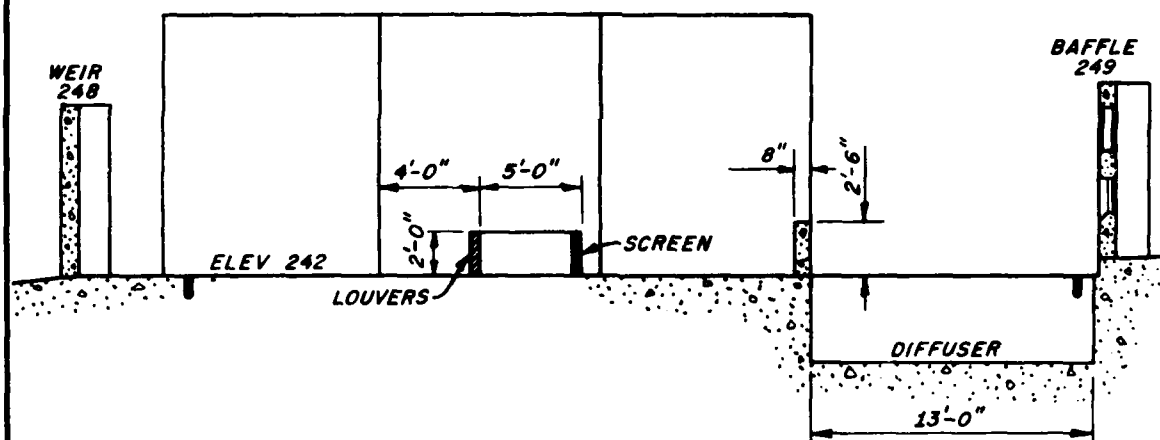
SECTION ALONG CENTER LINE
