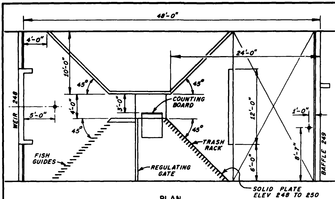
PLAN
