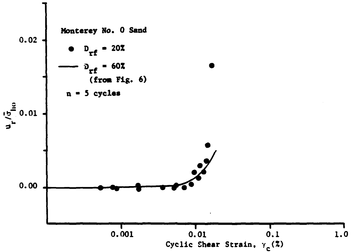
Figure 7 Effect of Relative Density on the Threshold Shear Strain ( k_c = 1.0 , T = 0 )
