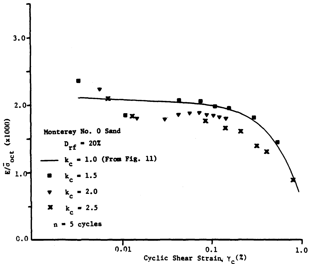
Figure 17 Effect of Anisotropic Consolidation on Normalized Young's Modulus ( D_{rf} = 20\% , T = 0 )
