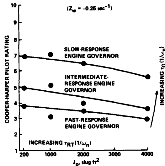
Figure 4. Effect of rotor inertia and engine governor.
