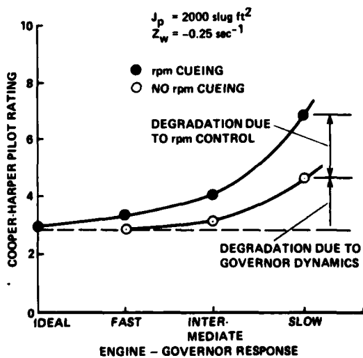
Figure 5. Effect of requiring rpm control.
