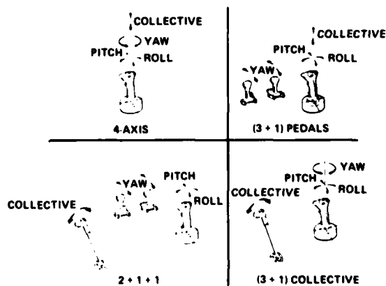
Figure 6. Controller configurations.
