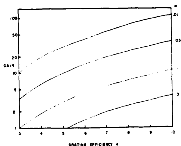
Fig. 12. Light gain when using two redistribution holograms.
