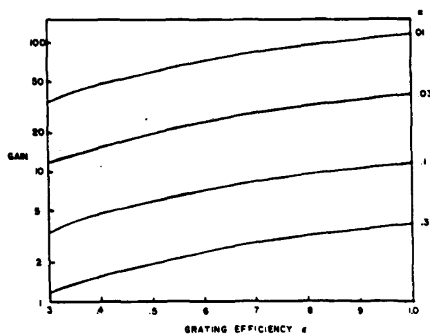
Fig. 11. Light gain when using one redistribution hologram.
