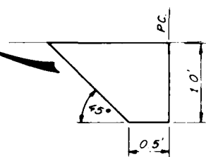
DEFLECTOR DETAIL
