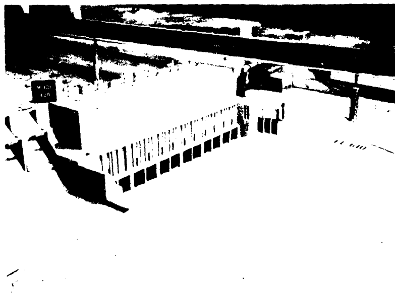
Powerhouse and adjacent pump intakes and fishway entrances
