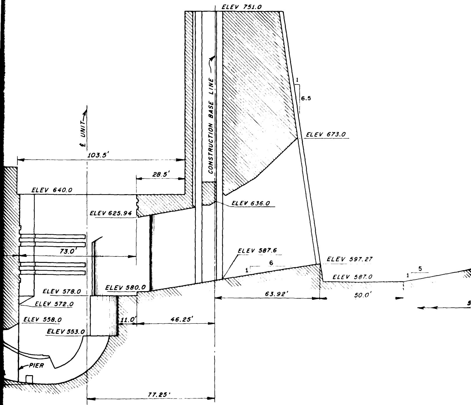
SECTION THROUGH UNIT
