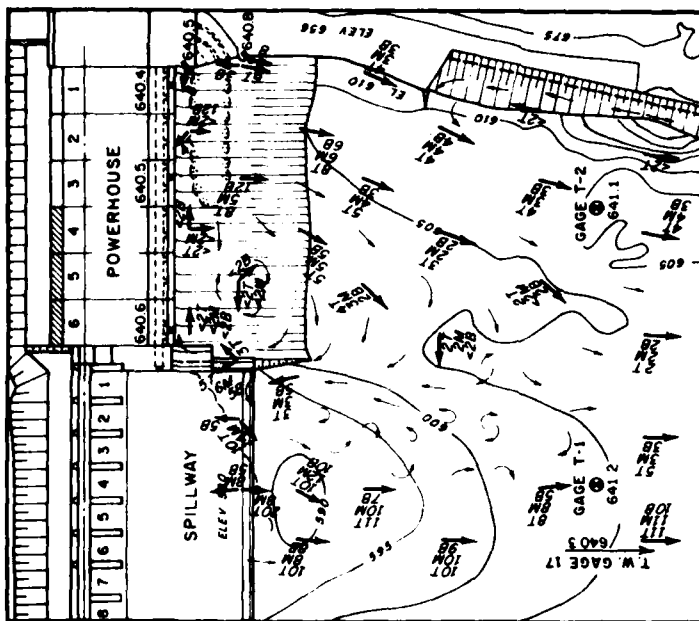
UNIFORM SPILLWAY OPERATION
