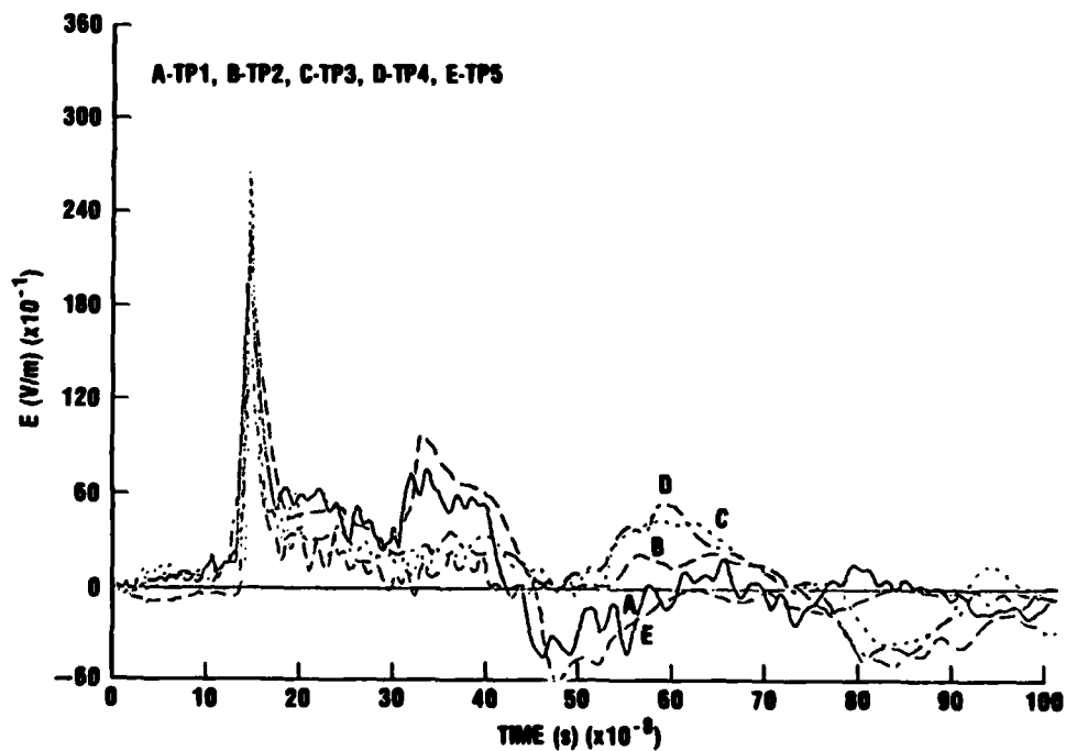
Figure 7. Transmitted electric field at TP1 to TP5 with \sigma = 0.02 mho/m and \epsilon_r = 15 .
